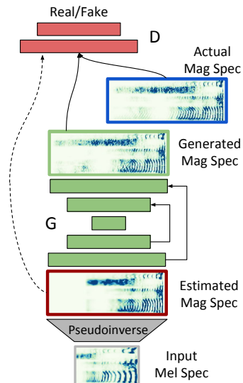
Figure 2: Adversarial Vocoder Model: The generator performs an image-to-image translation from the estimated magnitude spectrogram to the actual magnitude spectrogram guided by an adversarial loss from the discriminator and the L_1 distance between the generated and actual magnitude spectrogram
