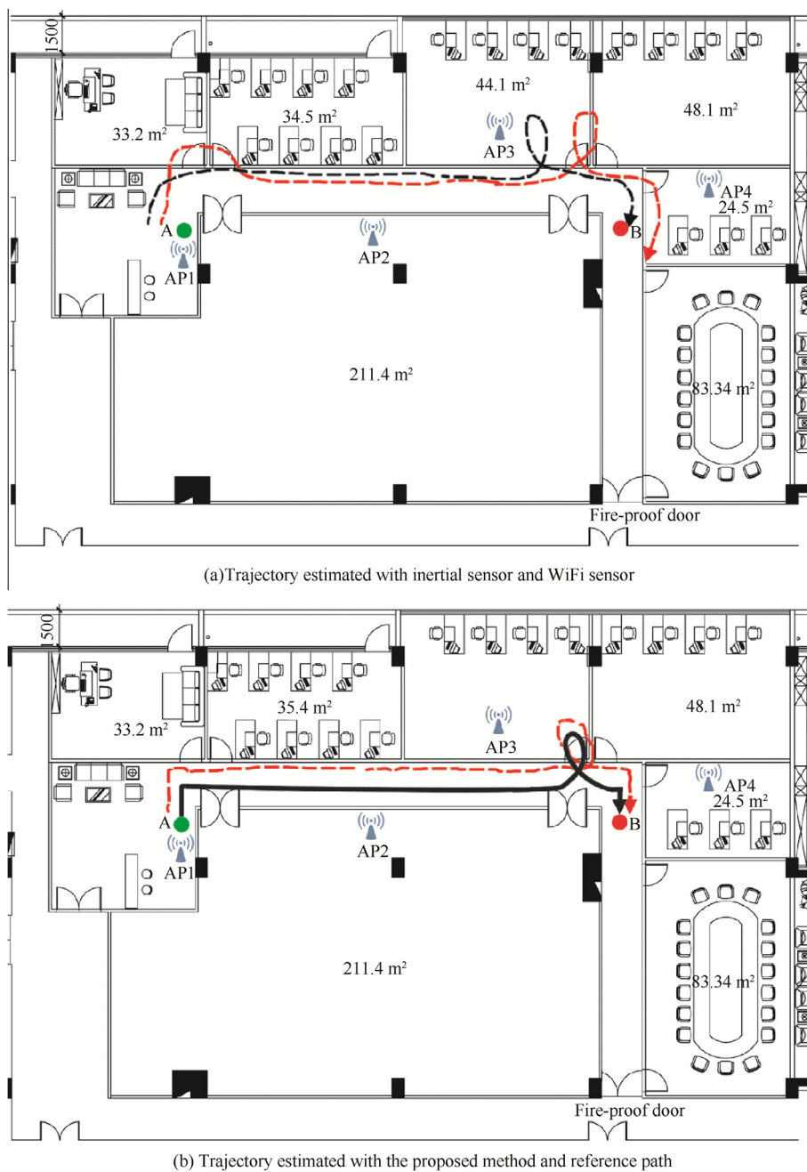
Fig. 9 Trajectory estimated.
