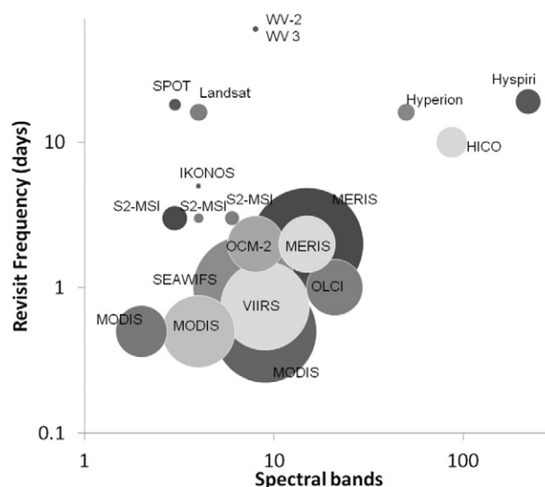
Fig. 5. The spectral (x-axis), temporal (y-axis), and spatial (size of the bubble) characteristics of satellite sensors commonly used for freshwater ecosystem measurements. Note: sensors that provide different spatial resolutions are plotted separately, and sensors with overlapping resolution characteristics are slightly jittered for graphing purposes.
