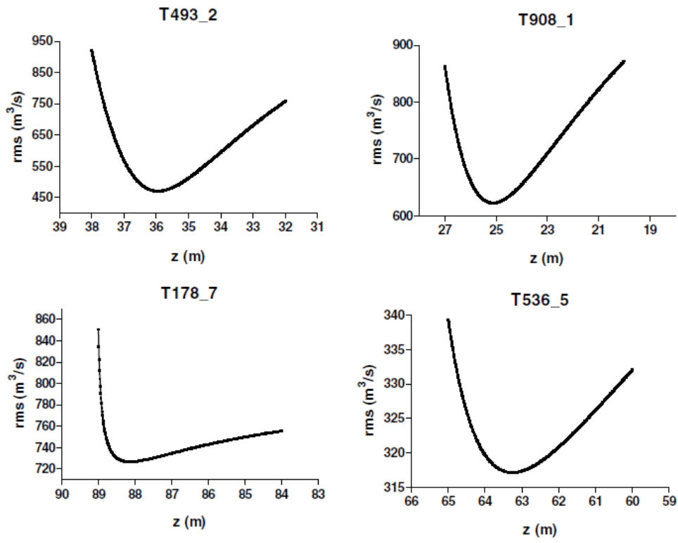
Figure 7 RMS evolution. Evolution of the RMS in discharge when the discharge–height pairs are fitted by a rating curve for successive values of the reference depth z .
