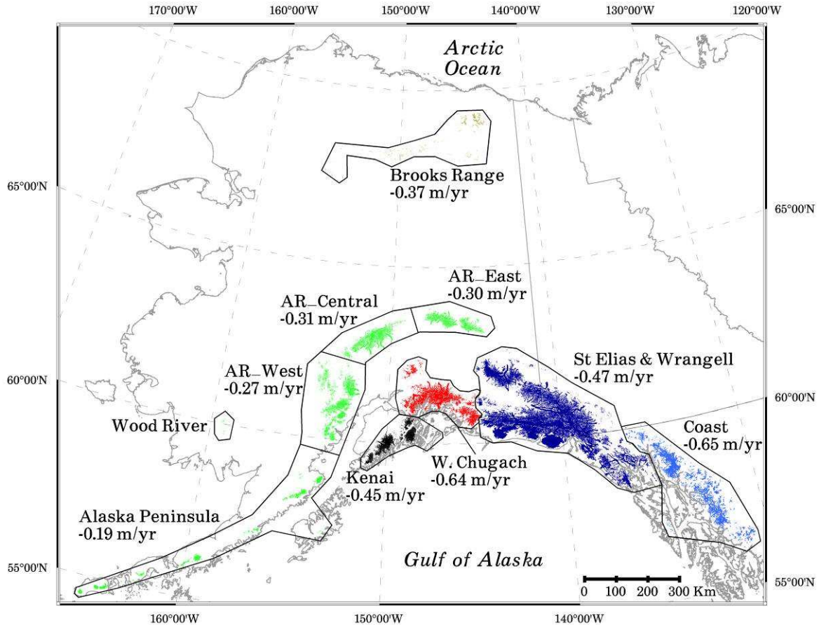
Figure 1: Regional area-average glacier mass balance in northwest North America between 1962 and 2006. The boundaries and names of the different glaciated regions follow those of Arendt et al. 2 , except that the Wrangell Mountains have been included in the St Elias Mountains. AR stands for Alaska Range.
