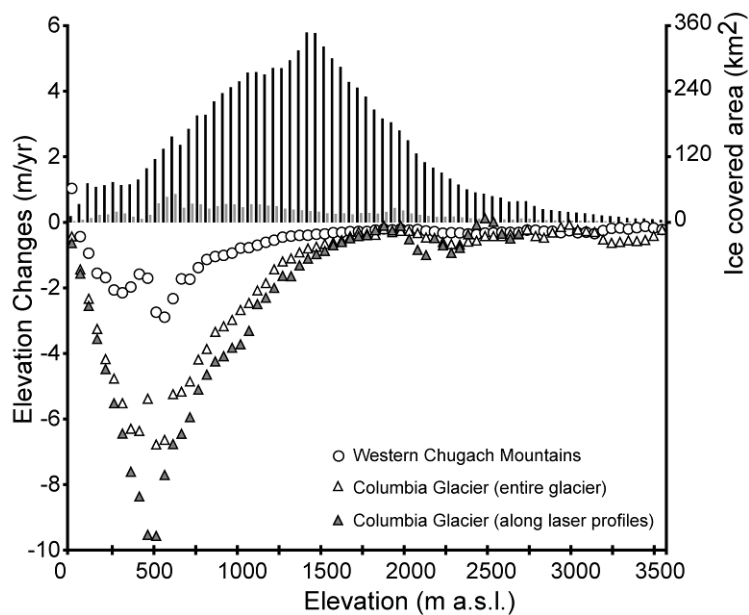
Figure 3: Hypsometry and rate of ice elevation change versus altitude in the Western Chugach Mountains. Upper panel, the hypsometry (distribution of ice-covered areas with altitude) is shown for the whole mountain range (9,149 km 2 ) and Columbia Glacier (1,066 km 2 ). Lower panel, 1957-2007 rate of ice elevation changes (averaged every 50-m elevation bins) extracted from the sequential DEM for the Western Chugach Mountains, the Columbia Glacier, and along the altimetric laser profiles (see Fig. 2) surveyed by Arendt et al. 2
