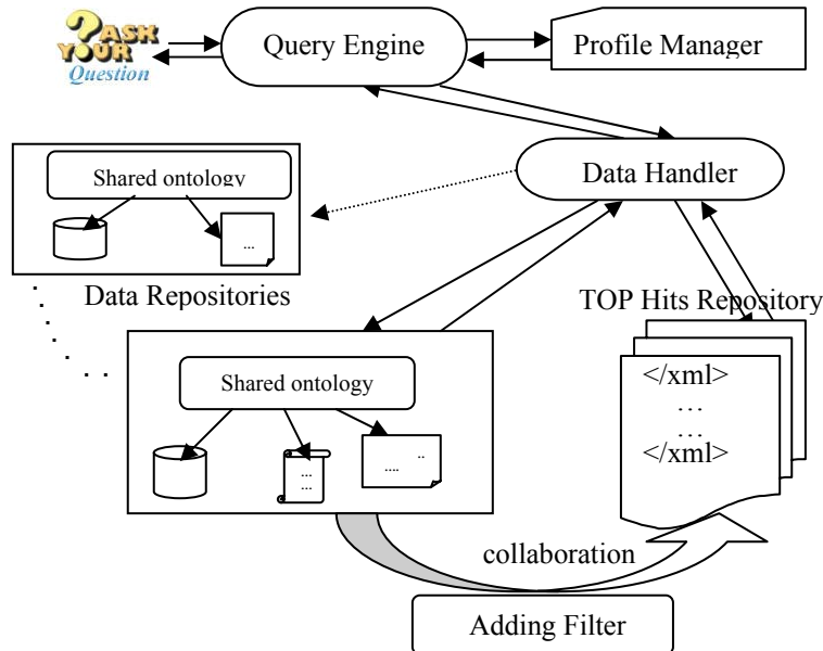
Fig. 1. A collaborative framework for location-based information management
