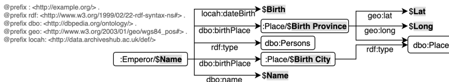
Fig. 2. RDF mapping for Roman emperors dataset. Bold text starting with $ references to a column in the dataset.
