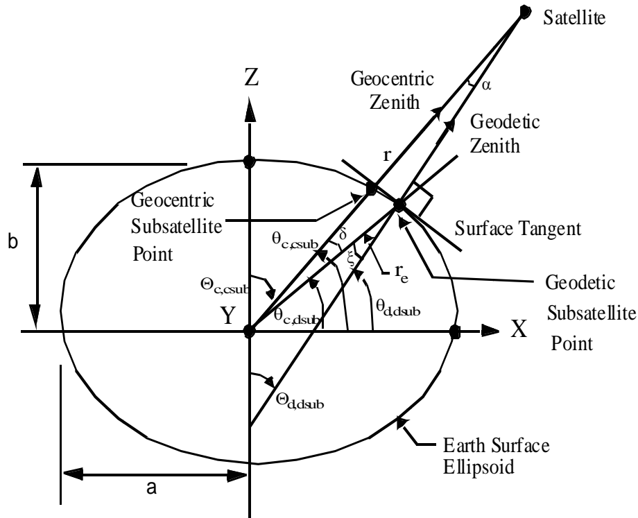
Figure 8-8. Subsatellite Point
