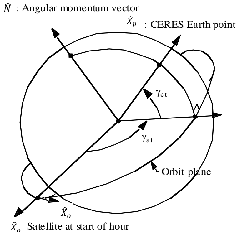
Figure 4-4. Along-track Angle
