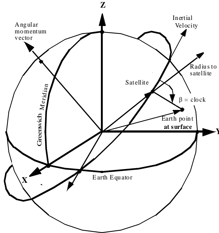
Figure 4-3. Clock Angle
