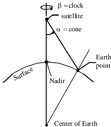
Figure 4-2. Cone and Clock Angles
