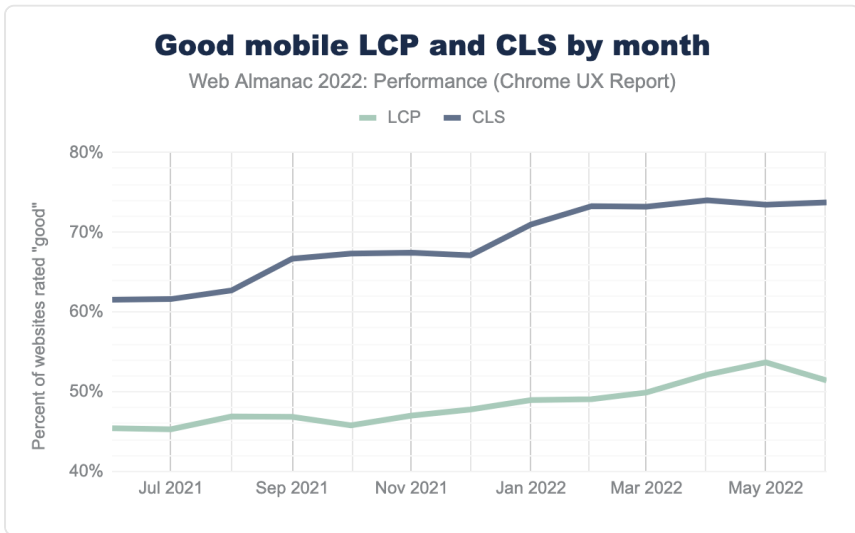
Figure 12.25. Monthly timeseries of the percent of websites having good mobile LCP and CLS.
