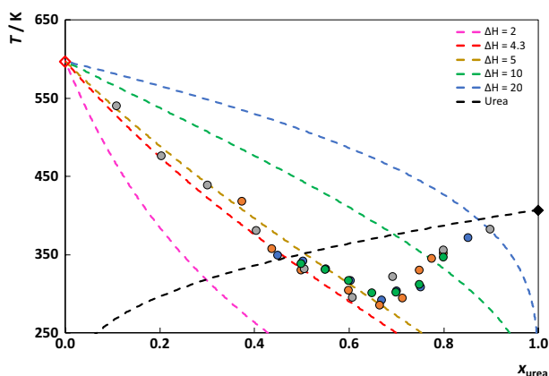
Fig. 5 Solid–liquid phase diagram of mixtures composed of choline chloride and urea. Full symbols represent experimental data: filled diamond, [59]; blue circle, [57]; orange circle, [9]; green circle, [58]; grey circle, unpublished data, and the empty diamond symbol, stands for the estimated T_{m,[Ch]Cl} = 597 \text{ K} [44]. Dotted lines correspond to ideal solubility curves calculated through Eq. 1 with T_{m,[Ch]Cl} = 597 \text{ K} [44] and \Delta_m C_p = 0 \text{ J}\cdot\text{mol}^{-1}\cdot\text{K}^{-1} . \Delta_m H is presented in units of \text{kJ}\cdot\text{mol}^{-1} (Color figure online)
