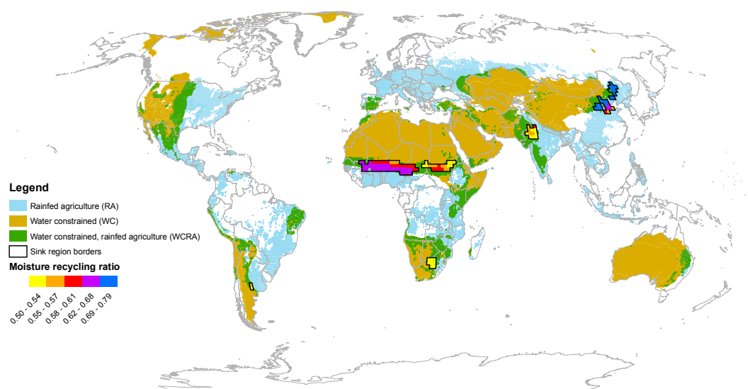
Fig. 2. Seven sink regions with rainfed agriculture, that are vulnerable to land cover change altering precipitation. The regions outlined in black are (a) located in water-constrained drylands (Portmann et al., 2010), (b) dominated by rainfed agriculture (Rockström and Karlberg, 2009), and (c) are dependent on terrestrial evaporation for more than 50 % of their growing season precipitation (van der Ent et al., 2010). Note that even though the sink regions are not green (which would indicate they are a WCRA region), they are in fact all water-constrained and dominated by rainfed agriculture.
