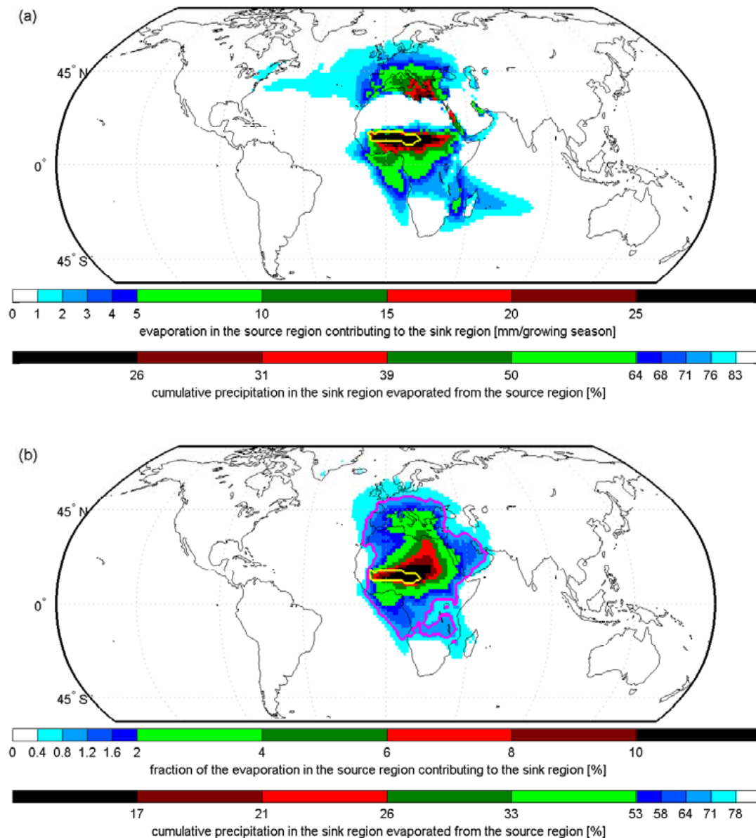
Fig. 3. Precipitationsheds of the West Sahel sink region: (a) The absolute precipitationsheds of the West Sahel sink region (yellow border), expressed in terms of absolute evaporation mm/growing season contributed to sink region precipitation; (b) The relative precipitationsheds of the West Sahel sink region (yellow border), expressed in terms of a fraction of the evaporation contributed to sink region precipitation. The second color scale in (a) and (b) indicates which percentage of the precipitation in the West Sahel region is generated within the area indicated by the corresponding colors. The pink border in (b) (= the gray border in Fig. 4) is the relative precipitationsheds for the West Sahel region (at 70 % contribution). The West Sahel sink region receives an average of 301 mm of precipitation per growing season. See Supplemental Figs. S2–S7 for the absolute and relative precipitationsheds of the other six sink regions.
