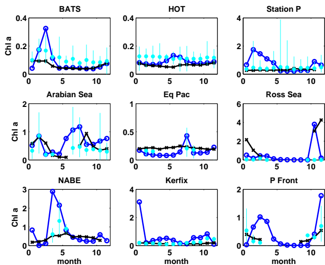
Figure 8. Comparison of monthly model Chl a ( \text{mgChl a m}^{-3} ) (dark blue) at nine sites (JGOFS data – Kleypas and Doney, 2001) with satellite (MODIS)-derived Chl a ( \text{mgChl a m}^{-3} ) (black) and in situ (light blue) data. In situ data show monthly mean of 0–15 m, with symbol and line indicating range of values. Locations of sites are shown in Fig. 1.
