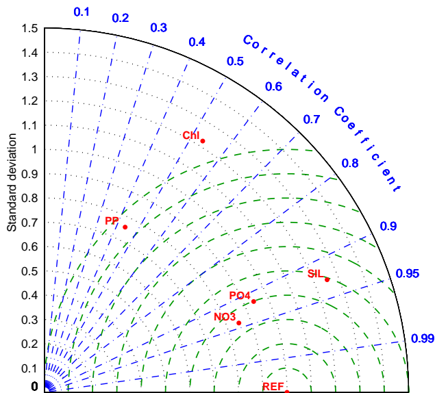
Figure 7. Taylor diagram showing correlation and normalized SD between annual mean modelled Chl a , primary production (PP), and macronutrients ( \text{NO}_3 , \text{PO}_4 , and silicic acid (SIL)). Satellite-derived products (Chl a from MODIS and primary production following Behrenfeld and Falkowski, 1997) and World Ocean Atlas (Garcia et al., 2006) nutrients. A perfect match would be a correlation of 1 (i.e. on the x axis) and normalized SD of 1: this point is shown as “REF”.
