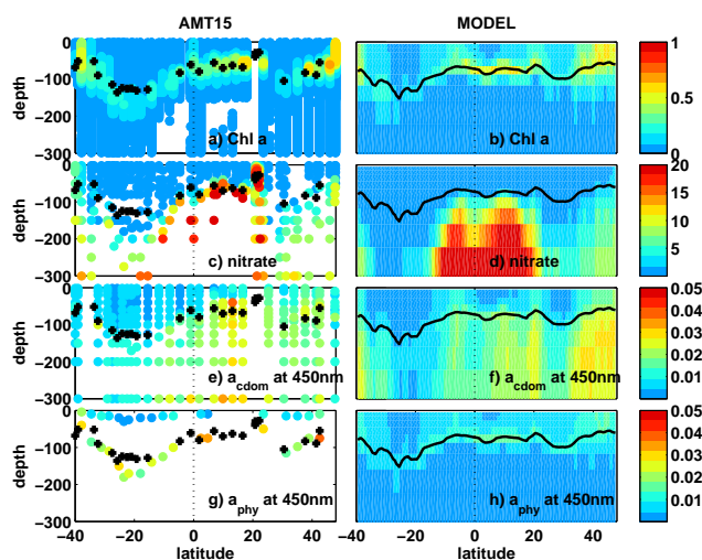
Figure 3. Comparison of model output (right column, October mean) with data collected during AMT-15 (left column, collected from late September to late October): (a, b) Chl a ( \text{mg Chl a m}^{-3} ), (c, d) nitrate ( \text{mmol N m}^{-3} ), (e, f) absorption by coloured dissolved matter ( a_{\text{CDOM}} ) ( \text{m}^{-1} ), and (g, h) absorption by phytoplankton ( a_{\text{phy}} ) ( \text{m}^{-1} ). The AMT-15 data are plotted as dots for each observation taken. Model data are presented across the whole transect. The black crosses indicate the depth where the total PAR is 1 % of the surface value in AMT-15. Model 1 % irradiance depth is shown as a black line. Transect location is shown in Fig. 2. (AMT-15 optical data – G. Moore, unpublished; CDOM – Stubbins et al., 2006).
