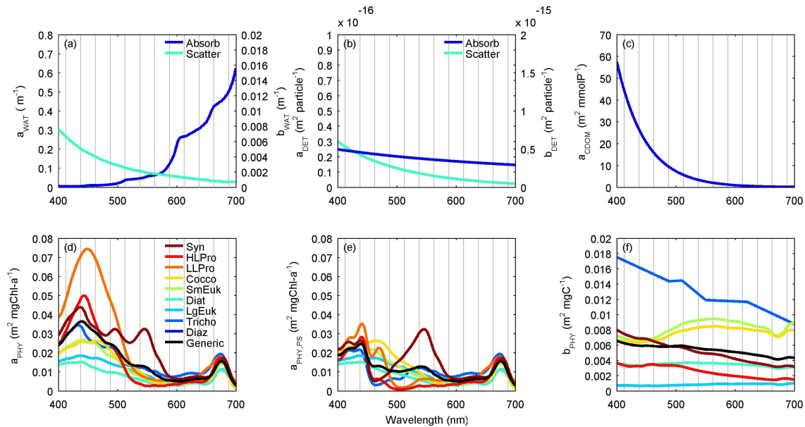
Figure 1. Spectra for (a) absorption and scattering by water molecules ( a_w , b_w , \text{m}^{-1} ); (b) particle-specific absorption and scattering by detritus ( a_{\text{det}}^{\text{part}} , b_{\text{det}}^{\text{part}} , \text{m}^2 \text{particle}^{-1} ); (c) CDOM-specific absorption by CDOM ( a_{\text{cdom}}^{\text{CDOM}} , \text{m}^2 (\text{mmolP})^{-1} ); (d) Chl a -specific total absorption by phytoplankton ( a_{\text{phy},j}^{\text{chl}} , \text{m}^2 (\text{mg Chl } a)^{-1} ); (e) Chl a -specific absorption by photosynthetic pigments ( a_{\text{ps},j}^{\text{chl}} , \text{m}^2 (\text{mg Chl } a)^{-1} ); and (f) biomass-specific scattering by phytoplankton ( b_{\text{phy},j}^{\text{C}} , \text{m}^2 (\text{mg C})^{-1} ). Details on data sources are included in the main text and Appendix Sect. C. The black line in (d–f) is the mean of the coloured lines (i.e. the mean spectrum). Spectra are shown here with 1 nm resolution for clarity; the model uses the average over the 25 nm bands (vertical grey lines).
