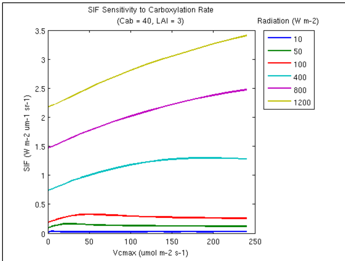
Fig. S2: Effect of incoming short wave radiation on the SIF- V_{cmax} sensitivity and for C3 plant. SIF is computed at the frequency 755 nm.
