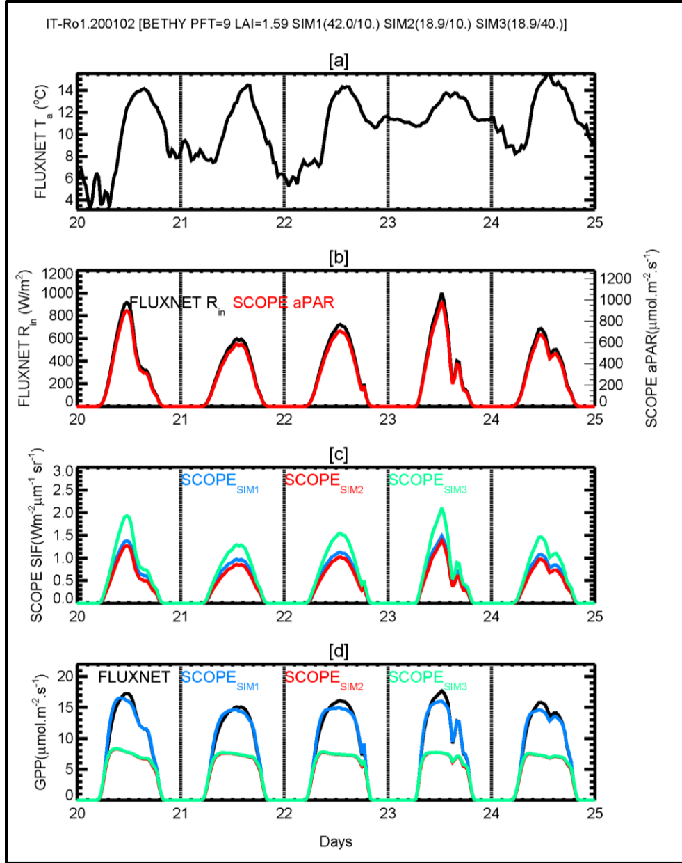
Fig. S5: SCOPE simulations of SIF, GPP, and aPAR from in situ measurements at Roccarespampani1 (acronym IT-Ro1 with longitude/latitude of 11.93/42.408) in Italy during 2001 over 20 to 25 February period. The graph a) presents the temporal variations of the observed temperature ( T_a ). Graph b) shows the temporal variations of both observed incoming short wave radiation R_{in} (black) and SCOPE simulated aPAR (red). Graphs c and d) display the simulated SIF and GPP by using two values of both V_{cmax} and C_{ab} (blue: SCOPE SIM1 : V_{cmax}/C_{ab} = 42 \mu\text{mol m}^{-2} \text{s}^{-1}/10 \mu\text{g cm}^{-2} ; red: SCOPE SIM2 : 18.9/10.; green: SCOPE SIM3 : 18.9/40.). The FLUXNET observed GPP is shown in graph d) and in black. The other SCOPE parameters are given in Table 1. The C3 plant is considered in SCOPE model. SIF is computed at the frequency 755 nm.
