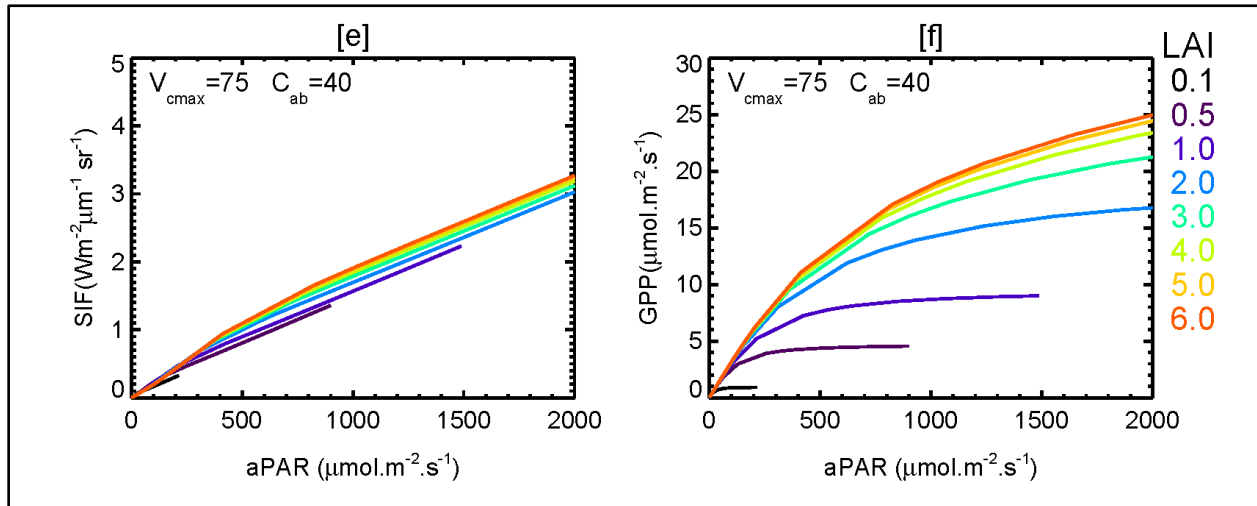
Fig. S1: The sensitivities of SCOPE fluorescence SIF (e) at the top of the canopy and GPP (f) of C3 plant to absorbed photosynthetically active radiation (aPAR) for several leaf area indices (LAI) are shown. The LAI values are shown on right hand side of the graph f). SIF is computed at the frequency 755 nm.
