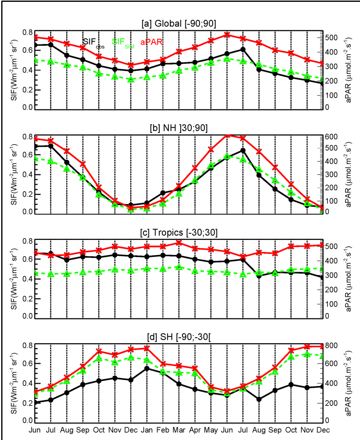
Fig. S9: Global (a) and regional (b to d) means of fluorescence SIF and absorbed photosynthetically active radiation (aPAR) over June 2009 to December 2010 period are shown. The satellite GOSAT based SIF ( SIF_{OBS} : black solid line with big dot), simulated SIF ( SIF_{SIM} : green dashed line with triangles), and the absorbed photosynthetically active radiation (aPAR: red solid line with crosses) are displayed. The CCDAS set up S4 (Table 3) is considered.
