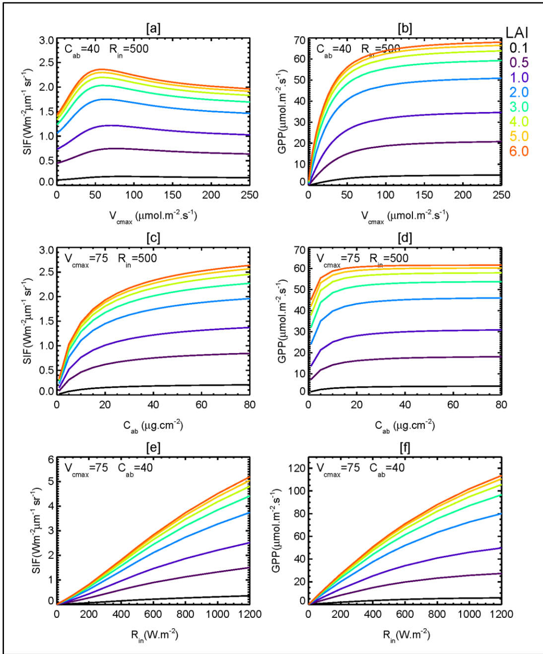
Fig. S3a: The sensitivities of SCOPE fluorescence (SIF) at the top of the canopy of C4 plant to the carboxylation maximum capacity ( V_{\text{cmax}} ), chlorophyll AB content ( C_{\text{ab}} ), and to broadband incoming shortwave radiation (0.4-2.5 \mu\text{m} ) ( R_{\text{in}} ) for several leaf area indices (LAI) are shown. Graphs a) and b) stand for SIF and GPP as function of V_{\text{cmax}} , respectively. The graphs c) and d) give the sensitivities of SIF and GPP to C_{\text{ab}} , respectively. The graphs e) and f) show SIF and GPP as a function of R_{\text{in}} , respectively. The LAI values are given on the top and the right hand side of the graph b). SIF is computed at the frequency 755 nm.
