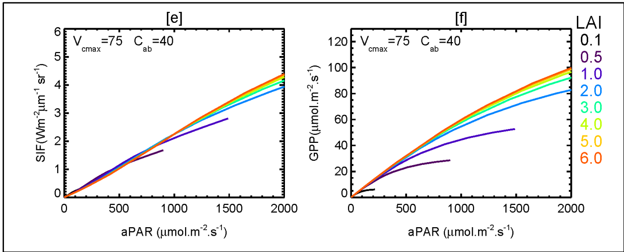
Fig. S3b: The sensitivities of SCOPE fluorescence SIF (e) at the top of the canopy and GPP (f) of C4 plant to absorbed photosynthetically active radiation (aPAR) for several leaf area indices (LAI) are shown. The LAI values are given on right hand side of the graph f). SIF is computed at the frequency 755 nm.
