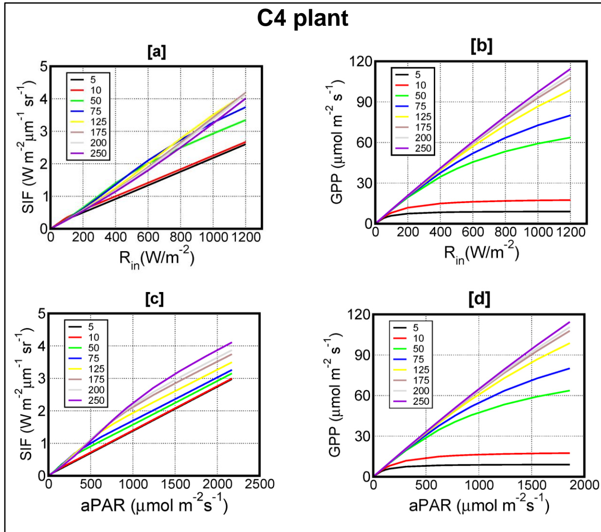
Fig. S4: The sensitivities of the SCOPE fluorescence SIF (a, c) and gross primary productivity (GPP) (b, d) to the incoming shortwave radiation ( R_{\text{in}} ) and absorbed photosynthetically active radiation (aPAR) and for several V_{\text{cmax}} are presented. LAI is set to 2. Results for a C4 plant are shown. The V_{\text{cmax}} values are shown in each graph. SIF is computed at the frequency 755 nm.
