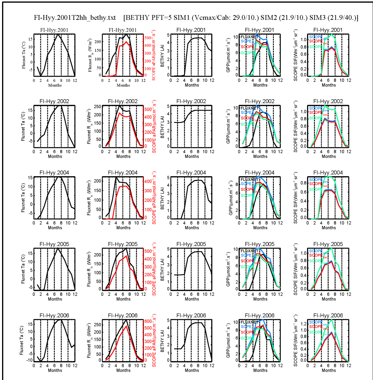
Fig. S6: Seasonal variations of FLUNET data (here temperature T_a , incoming short wave radiation at the top of the canopy R_{in} , and GPP) and SCOPE simulated quantities (aPAR, GPP, and SIF) at Hyytiala (acronym FI-Hyy and having longitude/latitude of 24.295^\circ/61.847^\circ ) by using BETHY monthly LAI relevant to the vegetation of the station. The simulated SIF and GPP are performed by using two values of both V_{cmax} and C_{ab} (blue: SCOPE SIM1 : V_{cmax}/C_{ab} = 29 \mu\text{mol m}^{-2} \text{s}^{-1}/10 \mu\text{g cm}^{-2} ; red: SCOPE SIM2 : 21.9/10; green: SCOPE SIM3 : 21.9/40). The observations are in black and simulations in colors. SIF is computed at the frequency 755 nm.
