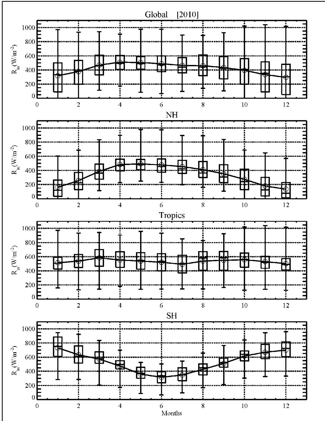
Fig. S8: Seasonal variations of the range of the incoming short wave radiation ( R_{in} ) used in the CCDAS simulations and for 2010 and at global and regional (Northern Hemisphere NH; Tropics; Southern Hemisphere SH) scales are shown. The minimum and maximum values of R_{in} for each month are shown. The boxes are delimited by the 25% and 75% percentiles. The median values are given by the horizontal line in the boxes. The mean values are given by the open circles
