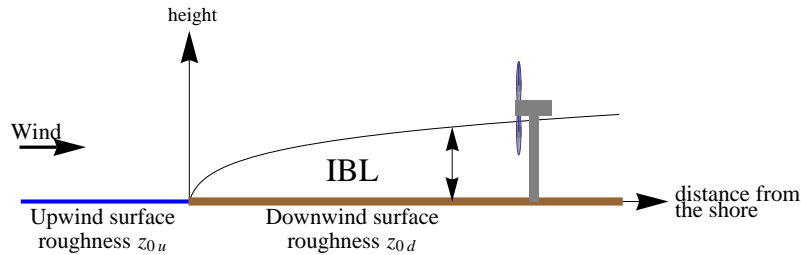
Figure 2.1: Conceptual model of an internal boundary layer
