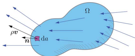
Fig. 2 A sketch of the mass current density field \rho \mathbf{v} (long arrows) flowing through an arbitrarily shaped, but fixed region \Omega (blue). Any infinitesimal area da (purple) is associated with an outward-pointing unit vector \mathbf{n} (short arrow) perpendicular to the local surface. The current flowing out through the area da is given by da times the projection \rho \mathbf{v} \cdot \mathbf{n} of the current density on the surface unit vector.
