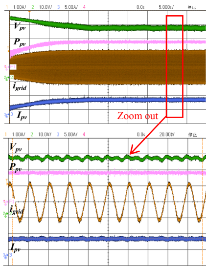
Fig. 13 MPPT key waveform @ P_{MP}=250\text{W} , V_{MP}=36\text{V}
