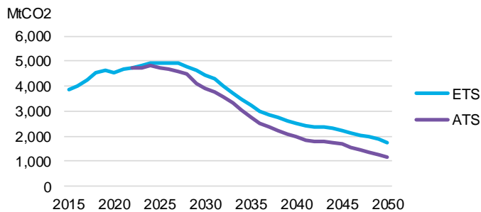
Figure 29: Power-sector emissions
