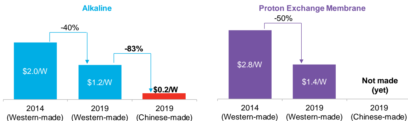
Figure 27: Benchmark system capex based on large-scale electrolyzers, 2014 and 2019
