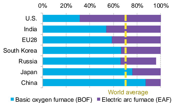
Figure 26: Comparison of steel furnace types, 2018
