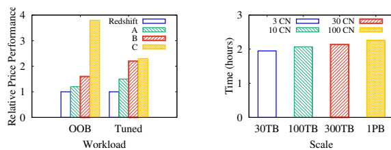
(a) Price-Performance comparison (b) Scaling TPC-DS from 30TB to 1PB
