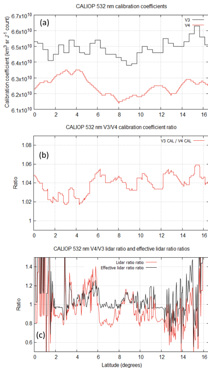
Figure 5: A comparison of CALIOP V4 and V3 532 nm calibration coefficients and lidar ratios around 07:18 UTC on 24 April 2010. (a) V3 and V4 532 nm calibration coefficients, (b) the ratio of V3 to V4 calibration, (c) the ratios of the V4 to V3 lidar ratios and effective lidar ratios.
