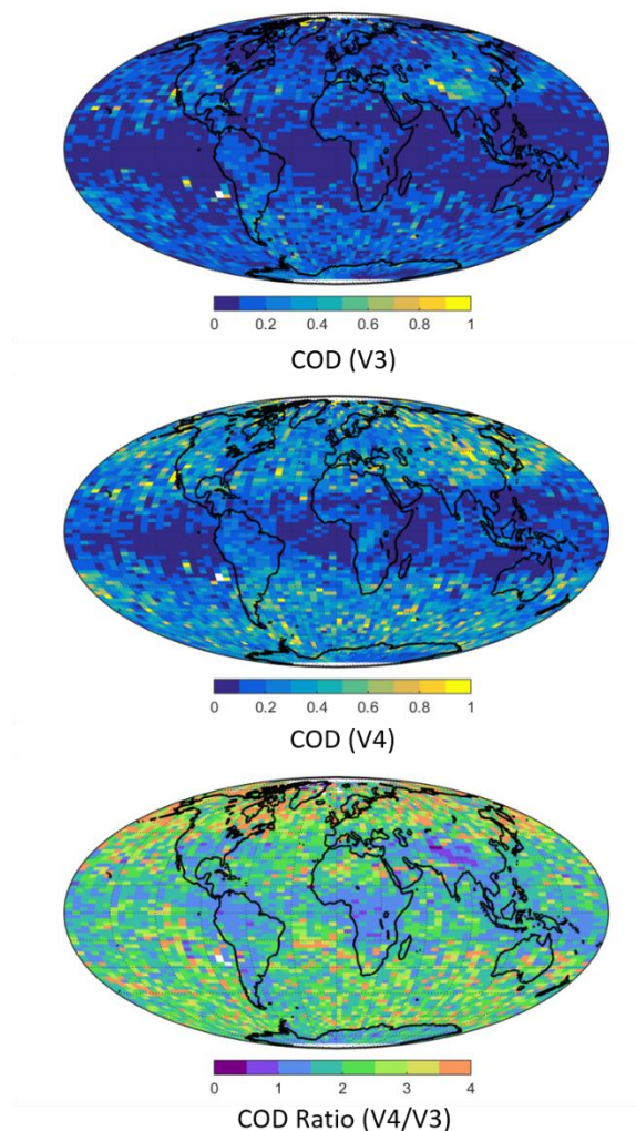
Figure 10: Median cloud optical depths (CODs) for semi-transparent, high-confidence nighttime ROI clouds for the period March to May 2010 inclusive, nighttime only. The area-weighted average optical depths from the maps are 0.137 for V3 (77,230,457 samples) and 0.266 for V4 (78,808,302 samples).
