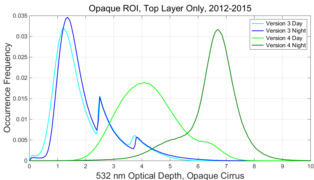
Figure 9: distributions of the apparent optical depths measured in opaque ROI clouds during 2012 – 2015 and processed using the V3 (blue) and V4 (green) algorithms.
