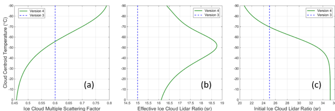
Figure 1: CALIOP ice cloud scattering parameters plotted as functions of cloud 532 nm attenuated backscatter centroid temperature, showing (a) multiple scattering factors, (b) effective lidar ratios (i.e., multiple scattering factor \times lidar ratio), and (c) lidar ratios for both V3 (dashed blue line) and V4 (solid green line). The multiple scattering factors and lidar ratios are sigmoid approximations to measured values reported in Garnier et al. (2015).
