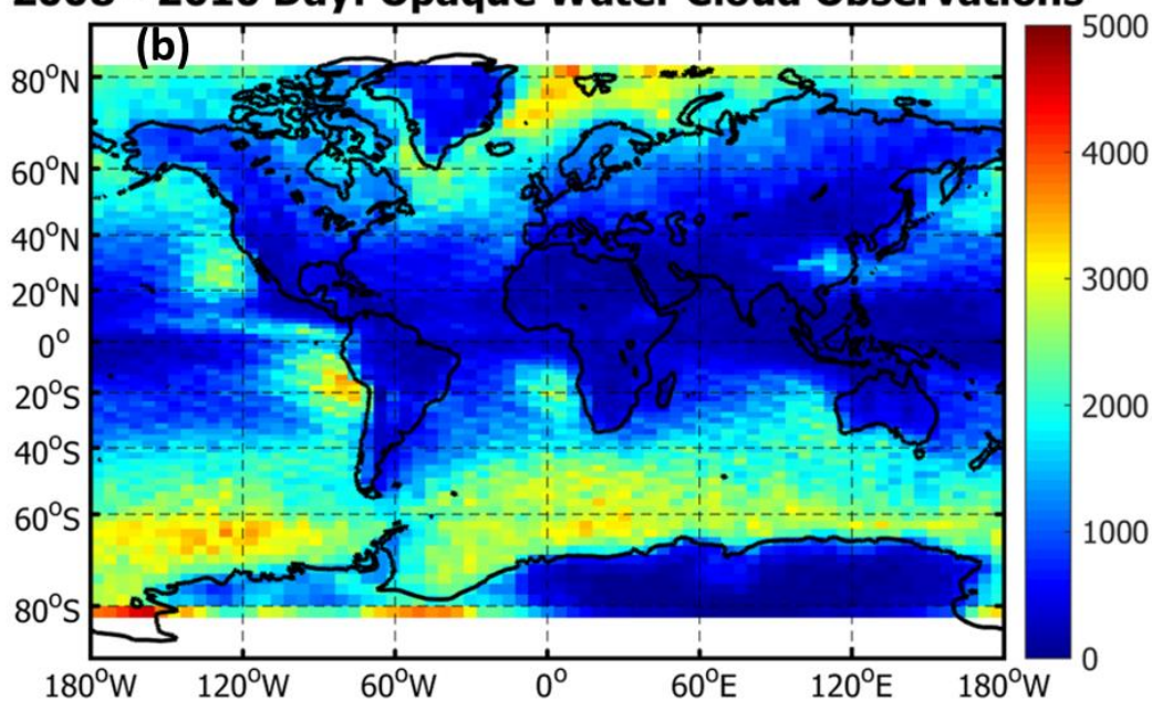
Figure 8: Mean global distribution of daytime opaque water clouds during 2008 – 2010; (a) 532 nm lidar ratios, (b) sample counts. Data have been filtered as described in the caption for Table 3.
