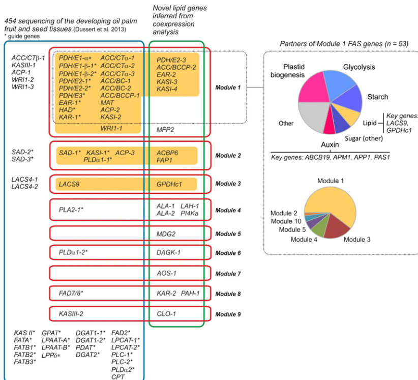
Figure 4. Lipid genes in the oil palm mesocarp coexpression network.
