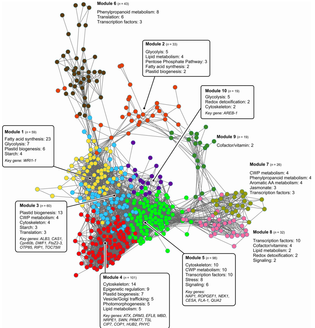
Figure 3. The oil palm mesocarp coexpression network.
