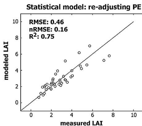
Fig. 6. Measured versus estimated (cross-validated) LAI in Majella National Park using statistical approaches with airborne HyMap spectra ( n=41 ). (left) Re-adjusting the polynomials against in situ data ( \text{PE}_{\text{re-adjust}} ): D -index with ( \lambda_1 : 846 nm, \lambda_2 : 1698 nm). (right) Identification of optimum index form, wavelengths and polynomials from experimental data (VI): R -index ( \lambda_1 : 543 nm, \lambda_2 : 1953 nm).
