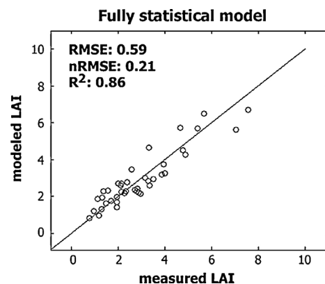
Fig. 6. Measured versus estimated (cross-validated) LAI in Majella National Park using statistical approaches with airborne HyMap spectra ( n=41 ). (left) Re-adjusting the polynomials against in situ data ( \text{PE}_{\text{re-adjust}} ): D -index with ( \lambda_1 : 846 nm, \lambda_2 : 1698 nm). (right) Identification of optimum index form, wavelengths and polynomials from experimental data (VI): R -index ( \lambda_1 : 543 nm, \lambda_2 : 1953 nm).
