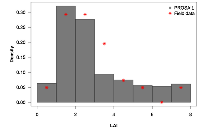
Fig. 5. Observed (dots) and modelled (bars) frequency distribution of LAI. The bars indicate the frequency distribution of PROSAIL derived LAI ( \text{m}^2 \text{m}^{-2} ) for a subset area of Majella National Park, Italy, using cleaned HyMap data and a LUT-based model inversion solutions. The dots indicate the distribution of field measurements.
