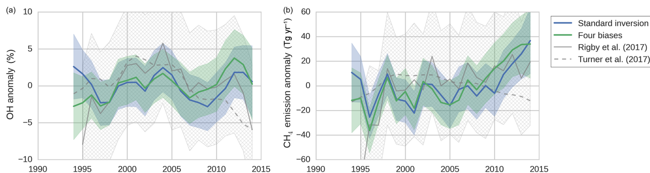
Figure 6. The results of two inversions of the two-box model: tropospheric OH anomalies (a) and CH 4 emission anomalies (b). In the standard inversion, we kept IH transport, NH / SH OH ratio, and stratospheric loss of MCF constant, and we used NOAA observations. In the second inversion, we implemented all four bias corrections instead (as described in Sect. 2.4). Both the mean anomalies and the 1-standard-deviation envelopes are shown, where anomalies were taken relative to the time-averaged mean in each respective ensemble member. Plotted in grey are the anomalies as derived by Rigby et al. (2017) (from the NOAA dataset) and by Turner et al. (2017) (from a combined NOAA and AGAGE dataset), adjusted so that they, too, average to zero. The 1-standard-deviation envelope from the Rigby et al. (2017) estimate is hatched in grey.
