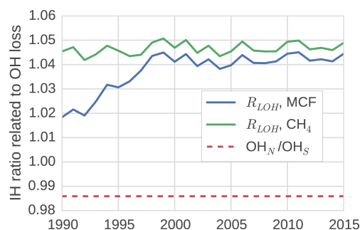
Figure 4. The ratio between tracer lifetime with respect to OH loss in the SH troposphere and NH troposphere (see Eq. 8). Additionally, the IH ratio in OH concentrations is shown.
