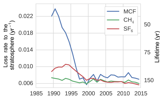
Figure 5. The tropospheric loss rate to the stratosphere, as derived from the TM5 simulations (see Sect. 2.2.2).
