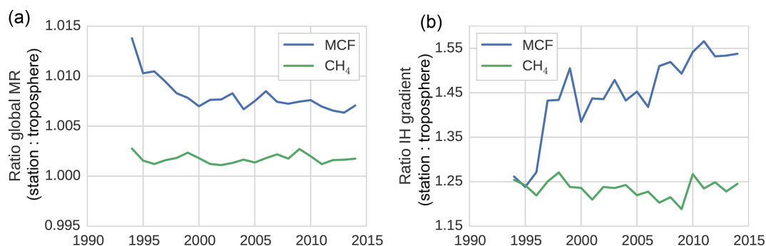
Figure 3. The surface sampling bias in the global mixing ratio (MR) (a) and in the IH gradient (b) of MCF and of \text{CH}_4 . The bias was quantified as the ratio between values derived from the NOAA surface sampling network and values derived from the full (TM5) troposphere. The biases were derived from 27 and 12 sites for \text{CH}_4 and for MCF, respectively. Figure 1 visualizes the impact of correcting for the sampling bias in real-world NOAA observations.
