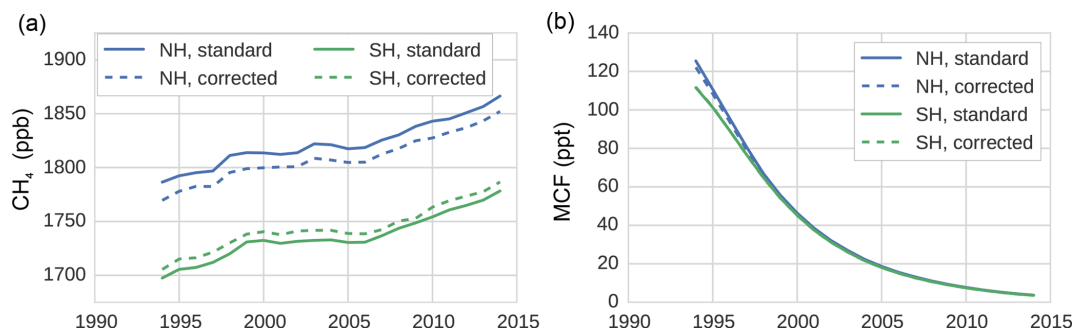
Figure 1. Hemispheric, annual mean time series of \text{CH}_4 (a) and MCF (b), as derived from the NOAA surface sampling network (for \text{CH}_4 , 27 sites were used; for MCF, 12 sites were used). Solid lines denote averages as derived directly from the NOAA surface sampling network (which are used in our standard inversion). Dashed lines denote the same time series, but those that are adjusted by correction factors that were derived from our TM5 simulations. The correction factors reflect the differences between hemispheric averages based on model-sampled observations and hemispheric averages derived from the full TM5 troposphere. Figure 3 shows the ratios between the standard and corrected time series.
