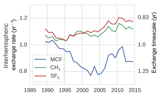
Figure 2. The IH exchange rate for MCF, \text{CH}_4 , and \text{SF}_6 , as derived from a TM5 simulation (see Sect. 2.2.2).
