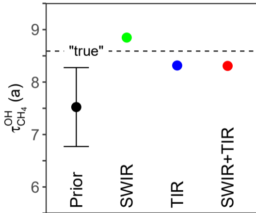
(b) Global OH concentration
