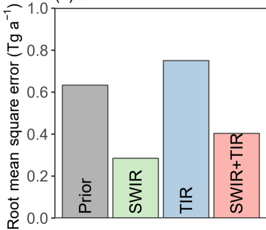
(a) Gridded methane emissions
