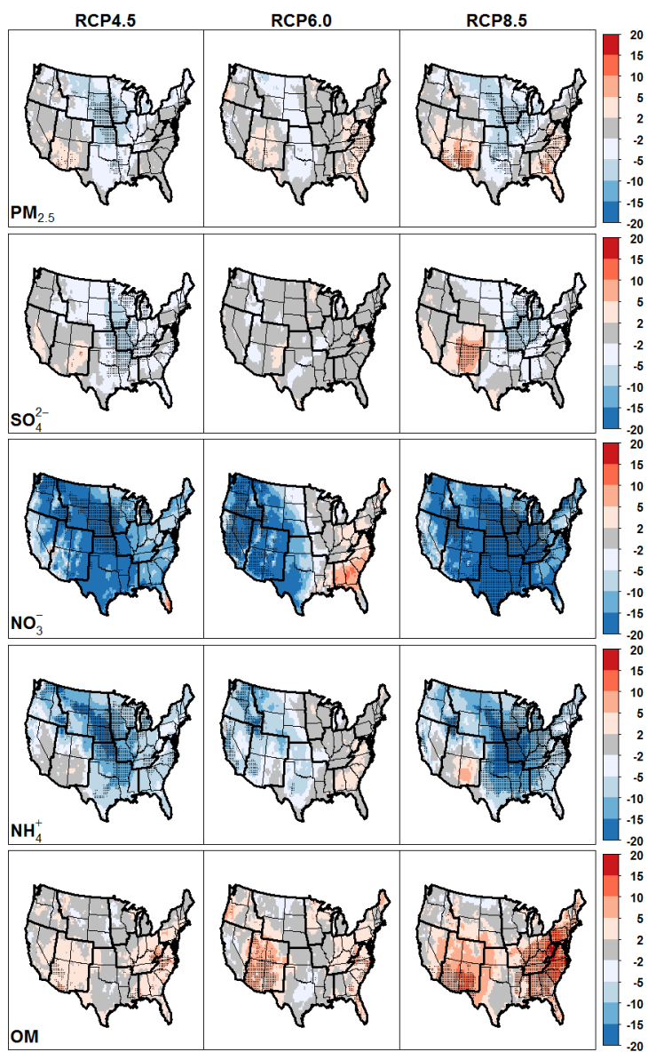
Figure S7: Projected relative changes (percent) in annual mean concentrations of total PM_{2.5} and principal PM_{2.5} components from 1995–2005 to 2025–2035 under RCP4.5, RCP6.0, and RCP8.5. Dark pixels show where differences are significant by Student's t-test ( p < 0.05 ).
