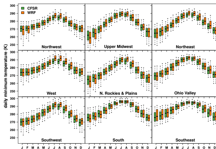
Figure S2: Monthly boxplots of daily minimum 2-m temperature simulated by downscaling CESM for the historical 1955–2005 period in comparison to CFSR for each of the U.S. climate regions shown in Figure 1. Boxes range from the 25th to 75th percentiles with the dark line denoting the median, and whiskers extend to 5th and 95th percentiles.
