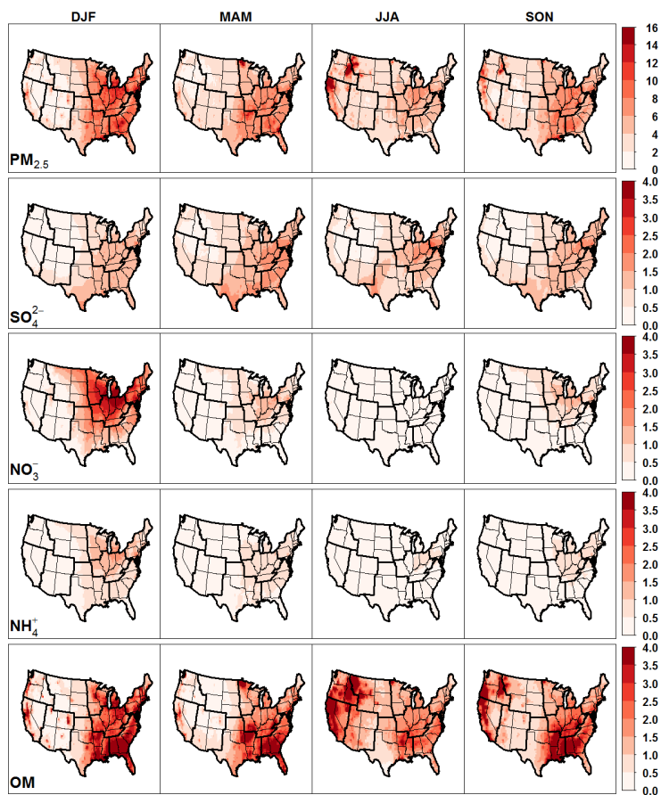
Figure S6: Seasonal mean PM 2.5 concentrations ( \mu\text{g m}^{-3} ) simulated for 1995–2005 using 2030 emissions projections provided in Table 1. (a) Total PM 2.5 ; (b) sulfate; (c) nitrate; (d) ammonium; and (e) organic matter.
