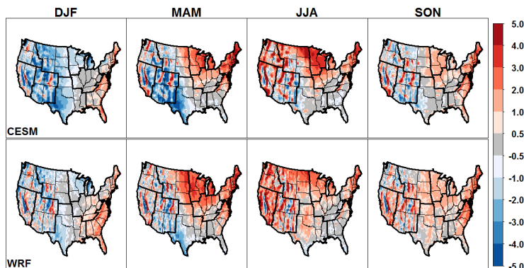
Figure S1: Seasonally averaged biases (K) in daily mean 2-m temperature compared to CFSR for 1955–2005. Top row shows biases in CESM fields interpolated to WRF grid; bottom row shows biases obtained after downscaling using WRF.
