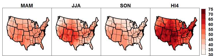
Figure S3: Maximum daily 8-h average (MDA8) O_3 mixing ratios (ppb) using meteorology down-scaled from CESM for the historical period 1955–2005 and 2030 anthropogenic emissions projections provided in Table 1. Values shown are 11-year averages of spring, summer, and autumn seasonal means as well as 4th-highest annual values.
