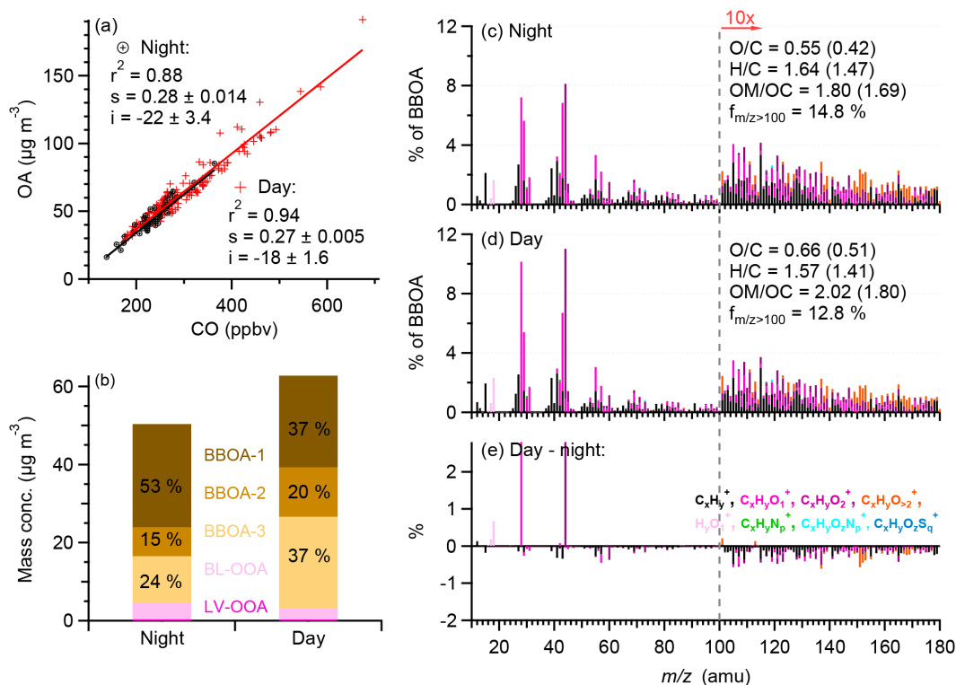
Figure 9. (a) OA vs. CO during 14 August at 20:00 to 16 August at 09:00 PDT with nighttime-transported plumes illustrated as black circles and daytime-transported plumes as red crosses. The orthogonal distance regression (ODR) results for the two plume types are shown with the 1\sigma uncertainties reported for the fit slopes ( s ) and intercepts ( i ); (b) a comparison of the average concentrations of five OA factors (stacked) between the nighttime- and daytime-transported plumes. The average mass fractions of the BBOAs to total OA mass in each plume type are reported; (c) average HRMS of total BBOA for the nighttime-transported plumes; (d) average HRMS of total BBOA for the daytime-transported plumes; and (e) difference BBOA HRMS between day and night plumes. The elemental ratios of BBOA calculated with the IA method are shown in the legends of panels (c) and (d), with those obtained using the AA method in parenthesis.
