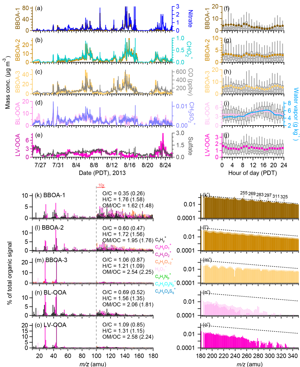
Figure 5. (a–e) Time series of OA factors and corresponding tracer compounds. Organic ions are in organic equivalent mass; (f–g) diurnal variations of OA factors (the whiskers above and below the boxes indicate the 90th and 10th percentiles, the upper and lower boundaries respectively indicate the 75th and 25th percentiles, the lines in the boxes indicate the median values, and the cross symbols indicate the mean values) with the diurnal cycle of mean water vapor in panel (i); (k–o) HRMS of OA factors colored by eight ion families at m/z < 180 , and (k'–o') UMR MS at m/z > 180 for each OA factor. The elemental ratios of each OA factor are shown in the legends of panels (k–o), with those obtained using the AA method in parenthesis.
