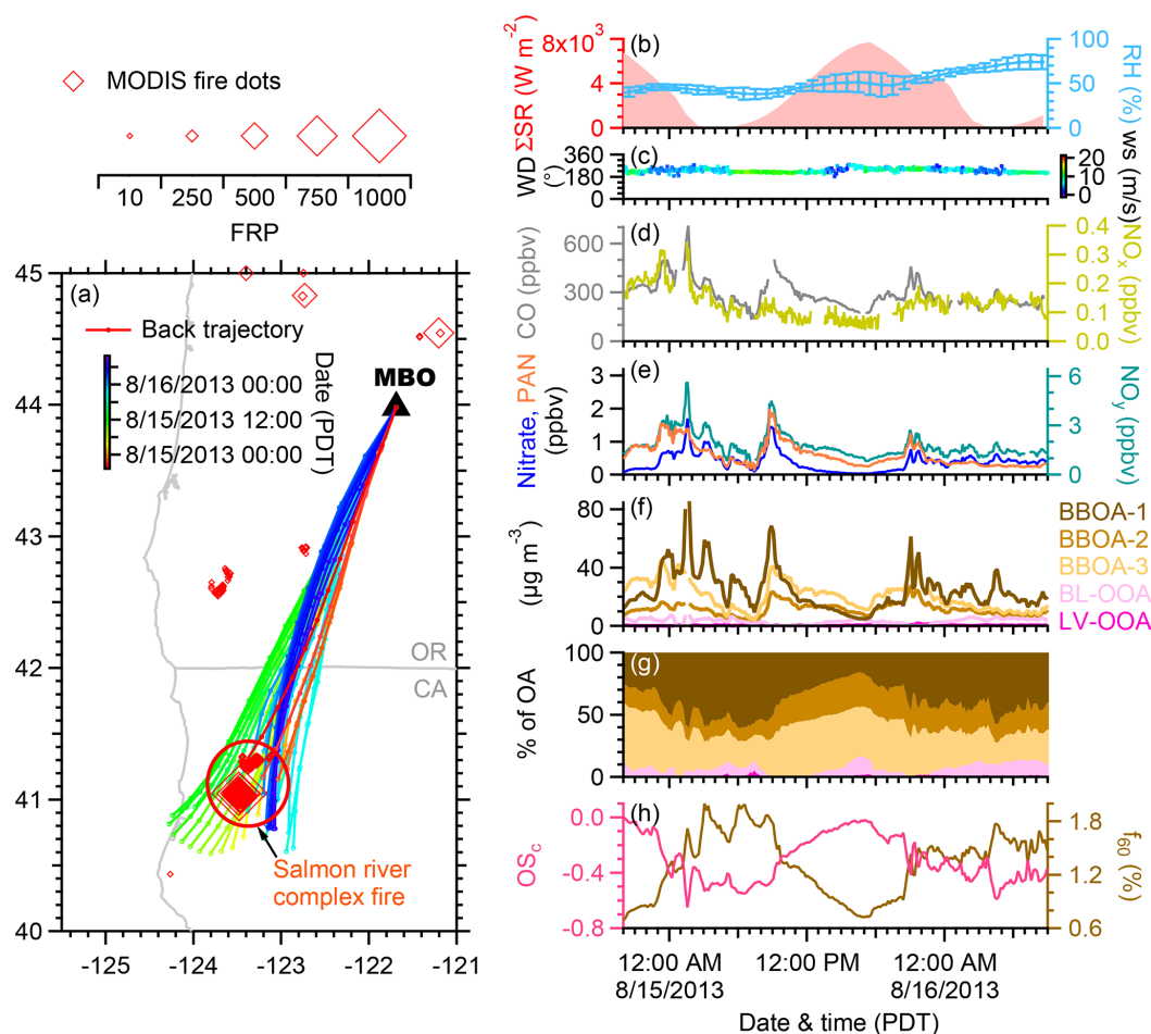
Figure 7. (a) Map of the Pacific Northwest with the location of MBO marked by a black triangle. Open diamonds represent MODIS satellite fire dots detected during 13–17 August 2013 and are sized by fire radiative power (FRP). Twelve-hour HYSPLIT back trajectories of air masses arriving at MBO from 14 August at 20:00 to 16 August at 09:00 PDT are colored by time of arrival at MBO. Markers indicate 1 h interval; (b) cumulative solar radiation ( \Sigma SR ) and average RH for each trajectory; (c) wind direction (WD) colored by wind speed (WS) measured at MBO; mixing ratios of (d) CO and NO_x ; mixing ratios of (e) nitrate, PAN, and NO_y ; (f) five OA factors; (g) OA composition; and (h) average carbon oxidation states and f_{60} of OA during the SRCF case study period.
