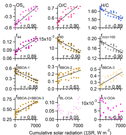
Figure 8. Aerosol chemistry parameters of total BBOA as a function of cumulative solar radiation for the Salmon River Complex fire case study. The Pearson's correlation coefficients ( r ) are reported.
