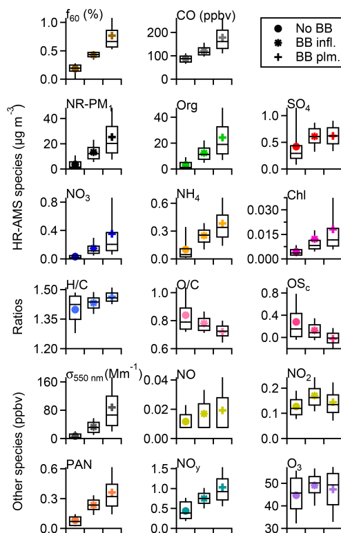
Figure 3. Box plots that compare f_{60} values, CO mixing ratios, NR-PM 1 species concentrations, OA elemental ratios, carbon oxidation states ( OS_c ), \sigma_{550\text{ nm}} , and mixing ratios of trace gases among three aerosol regimes (No BB, BB Infl, and BB Plm). The whiskers indicate the 90th and 10th percentiles, the upper and lower boundaries respectively indicate the 75th and 25th percentiles, the lines in the boxes indicate the median values, and the markers indicate the mean values.
