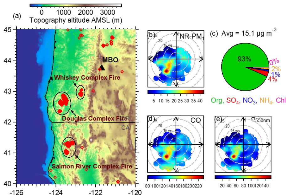
Figure 1. (a) Map with MBO (black solid triangle) and wildfires detected by MODIS (red open diamonds) in the US Pacific Northwest from 25 July to 25 August 2013. Three fire complexes – Whiskey Complex fire (WCF), Douglas Complex fire (DCF), and Salmon River Complex fire (SRCF) – are highlighted with black circles. Bivariate polar plots of (b) NR-PM 1 concentrations (in \mu\text{g m}^{-3} ), (d) submicrometer aerosol light scattering at 550 nm ( \sigma_{550\text{nm}} in \text{Mm}^{-1} ), and (e) CO mixing ratio (in ppbv) during the sampling period. (c) Average NR-PM 1 composition for the sampling period.
