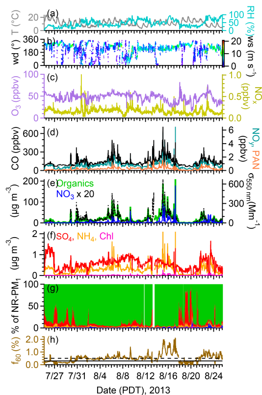
Figure 2. Time series of (a) temperature ( T ) and relative humidity (RH); (b) wind direction (WD) colored by wind speed (WS); (c) mixing ratios of O 3 and NO x ; (d) mixing ratios of CO, NO y , and PAN; (e, f) mass concentrations of NR-PM 1 species and \sigma_{550\text{nm}} in STP ( T = 273 K, P = 1013.25 hPa); (g) NR-PM 1 composition; and (h) f_{60} ( = \text{C}_2\text{H}_4\text{O}_2^+ / \text{OA} ). The solid and broken lines in panel (h) indicate f_{60} = 0.3 % and f_{60} = 0.5 %, respectively.
