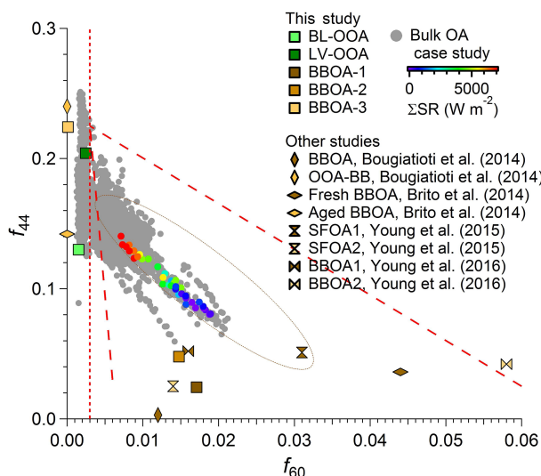
Figure 4. Scatterplot of f_{44} vs. f_{60} . The grey markers correspond to the measured OA during this study, and the SRCF case study data are colored by cumulative solar radiation ( \Sigma SR). In addition, the five OA factors identified in this study are shown as solid squares, and the BBOA factors reported in the literature where multiple BBOA factors were derived are shown with different markers. The dashed red lines denote f_{60} = 0.003 and the boundaries set for BBOA (Ortega et al., 2013). The brown oval encompasses ARCTAS fire plumes sampled above the North America continent (Cubison et al., 2011).
