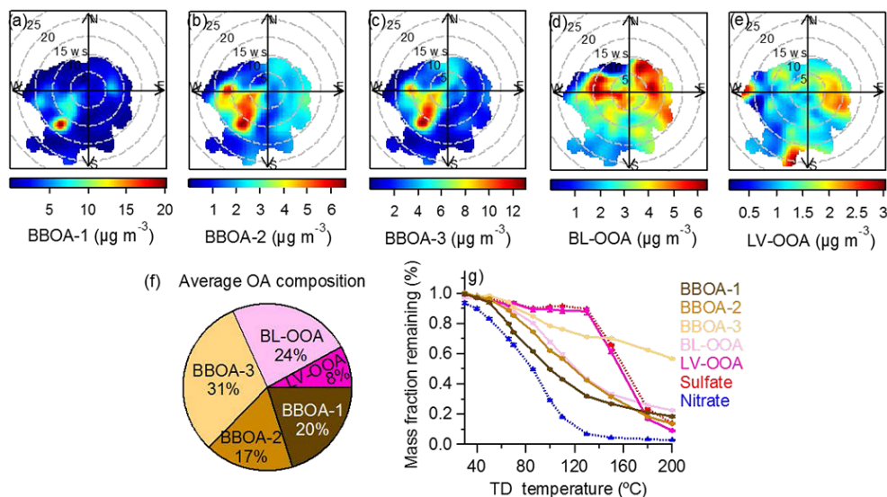
Figure 6. (a–e) Bivariate polar plots that illustrate the variations of the concentrations of each OA factor as a function of wind speed ( \text{m s}^{-1} ) and wind direction; (f) average OA composition during the sampling period; and (g) volatility profiles of OA factors, sulfate, and nitrate, with error bars showing the standard deviation of the calculated slope, i.e., mass fraction remaining.
