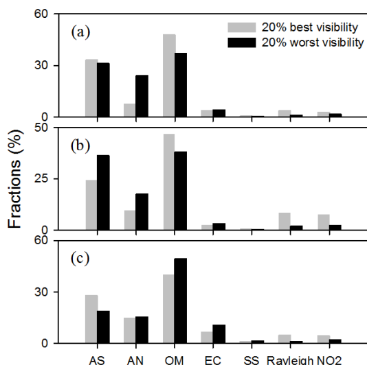
Figure 5. Relative contributions of various chemical components in PM 2.5 (ammonium sulfate (AS), ammonium nitrate (AN), OM, and EC) to the total light extinction under 20 % best and 20 % worst visibility conditions during the first (a), second (b), and third (c) haze events.
