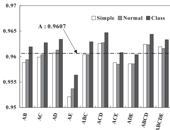
Figure 4: 11-point accuracy: A included
