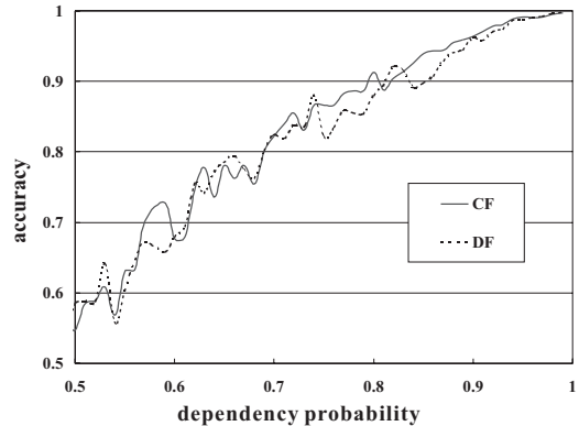
Figure 8: P-A curves: +KNP
