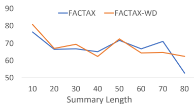
Figure 2: Accuracy of FACTAX methods for different summary lengths using ChatGPT.
