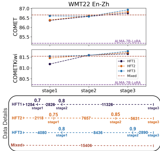
Figure 6: Robustness against threshold \mu and \nu . HFT1: (\mu, \nu) = (0.7, 0.8) , HFT2: (\mu, \nu) = (0.75, 0.85) , and HFT3: (\mu, \nu) = (0.8, 0.9) . Mixed denotes mixed training. ALMA-7B-LoRA is the model to refine.
