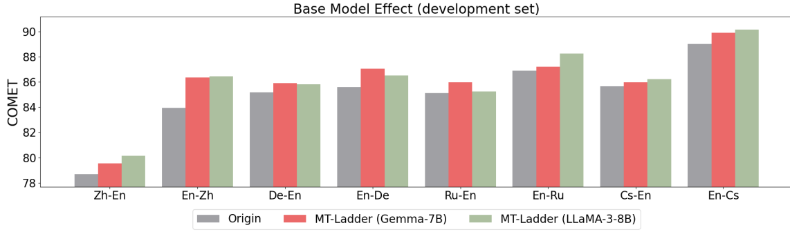
Figure 10: COMET scores of using different models as the base model of MT-Ladder. Origin denotes ALMA-7B-LoRA translation.
