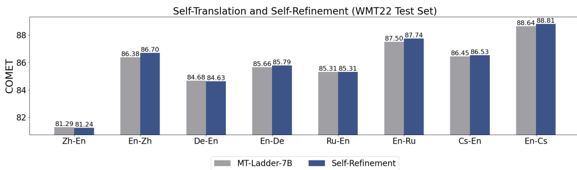
Figure 15: COMET scores for Self-translation and Self-refinement with MT-Ladder-7B. Self-Refinement denotes MT-Ladder-7B refines its original translation.
