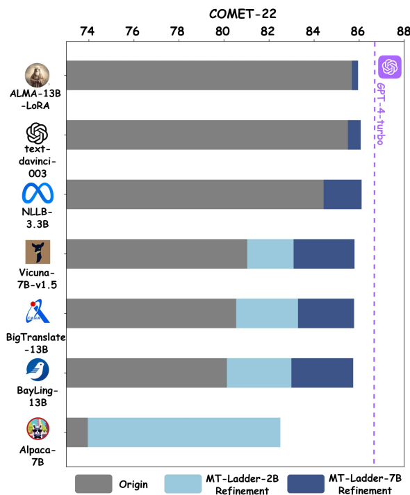
Figure 1: The average translation quality improvements across 8 translation directions on WMT22 test set (Zh↔En, De↔En, En↔Ru, En↔Cs) using MT-Ladder-2B or 7B. The metric scores are calculated by COMET-22 ( wmt22-comet-da ) (Rei et al., 2020).
