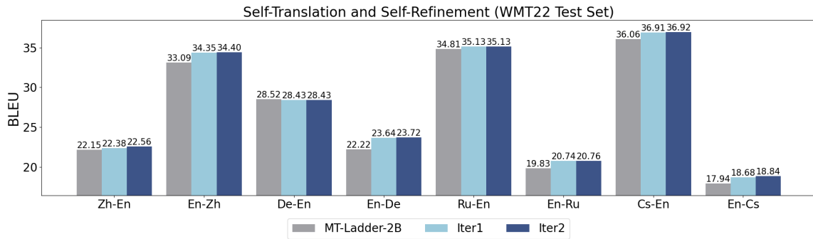
Figure 12: BLEU scores for Self-translation and Self-refinement. Iter1 denotes MT-Ladder-2B refines its original translation. Iter2 denotes MT-Ladder-2B refines the MT-Ladder-2B edited translation in Iter1 .
