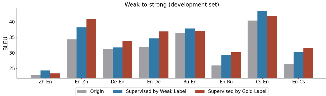
Figure 11: Weak-to-strong BLEU scores. We fine-tune Gemma-7B using different references as the label to refine the development set. Origin denotes ALMA-7B-LoRA translation. Blue represents using ALMA-7B-LoRA as references . Red represents using the gold as references .
