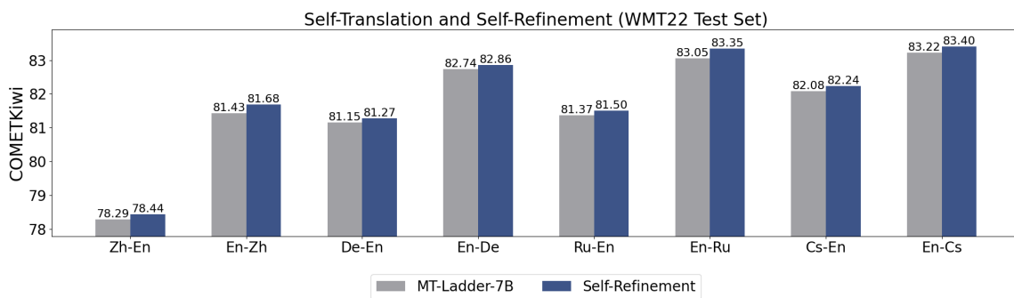
Figure 16: COMETKiwi scores for Self-translation and Self-refinement with MT-Ladder-7B. Self-Refinement denotes MT-Ladder-7B post-edits its original translation.
