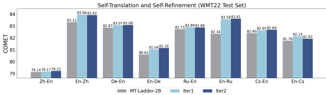
Figure 8: Self-translation and Self-refinement. MT-Ladder-2B represents performing direct translation with prompt \mathcal{P}_D , demonstrating translation capabilities comparable to 7B and 13B LLM-based translators. Iter1 denotes MT-Ladder-2B refining its original translation. Iter2 denotes MT-Ladder-2B refining the translation from Iter1 .
