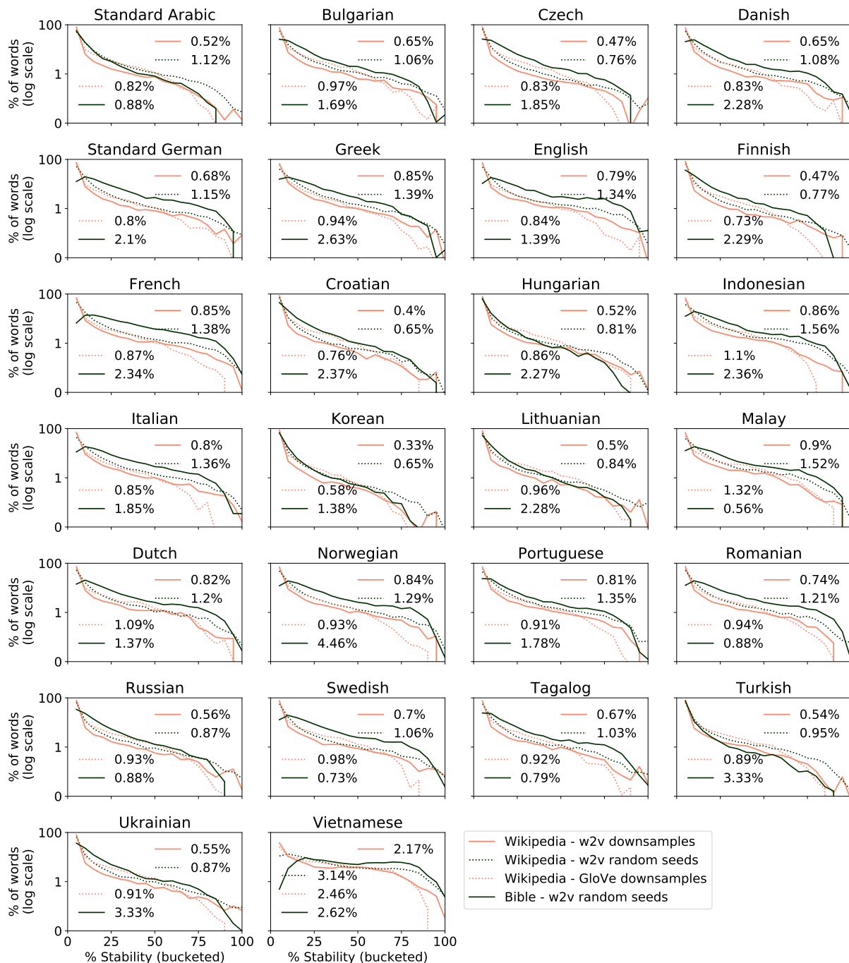
Figure 2: Percentage of words that occur in each stability bucket for four different methods, three on Wikipedia and one on the Bible. The 26 languages in common are shown here. The average stability for each method is shown on the individual graphs.
