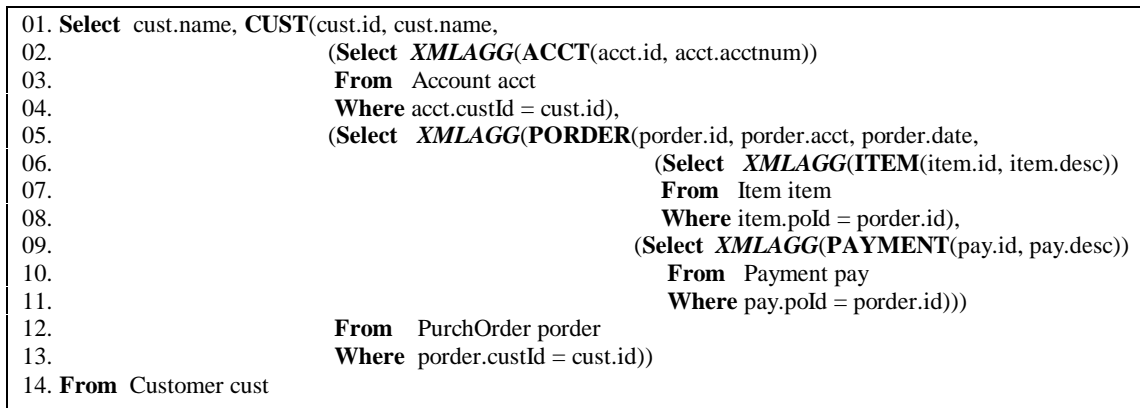
Figure 3: SQL Query to Construct XML Documents from Relational Data
