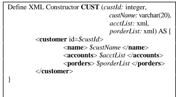
Figure 4: Definition of an XML Constructor
