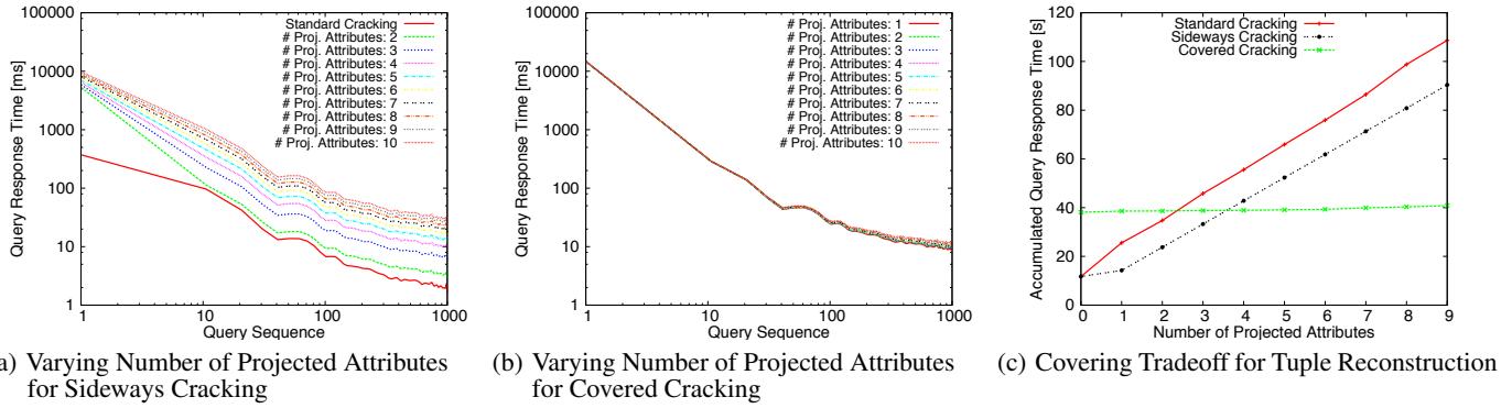
Figure 6: Comparing Tuple Reconstruction Cost of Standard, Sideways, and Covered Cracking
