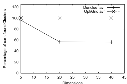
Figure 11: Dependency on the Dimensionality
