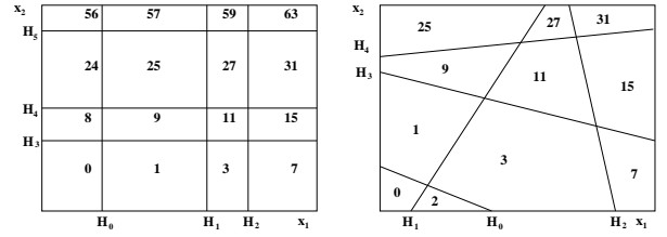
(a) regular (b) irregular Figure 3: Examples of 2-dimensional Grids
