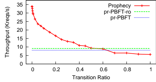
Figure 9: Throughput of reads of a 1-byte webpage to Apache webserver for proxied systems.
