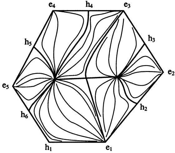
e_1 - e_5 are elliptic vertices, h_1 is a hyperbolic vertex, h_2 - h_6 are pseudovertices
