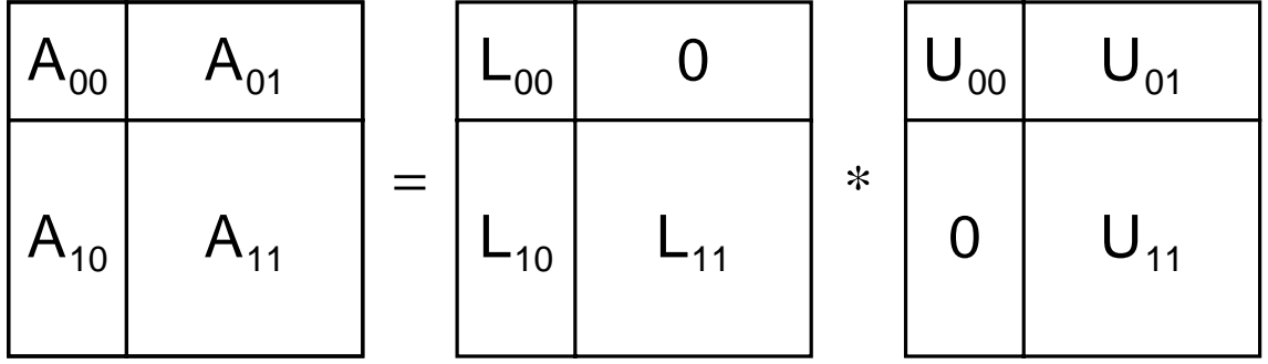
Figure 5: Block LU factorization of the partitioned matrix A . A_{00} is r \times r , A_{01} is r \times (N - r) , A_{10} is (M - r) \times r , and A_{11} is (M - r) \times (N - r) . L_{00} and L_{11} are lower triangular matrices with 1's on the main diagonal, and U_{00} and U_{11} are upper triangular matrices.
