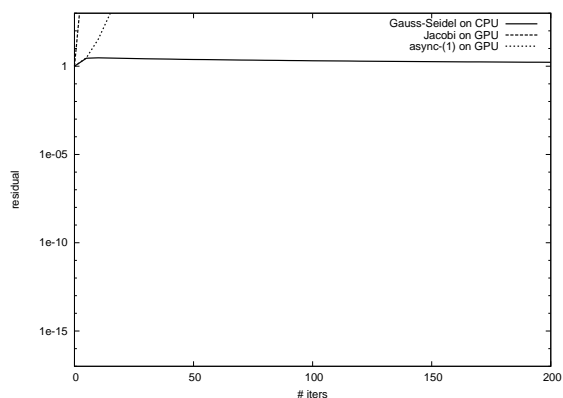
Figure 8: Convergence behavior of test matrix S1RMT3M1
