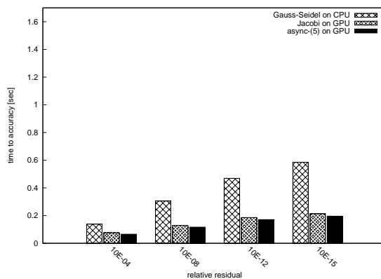
Figure 17: Time to solution for CHEM97ZTZ.
