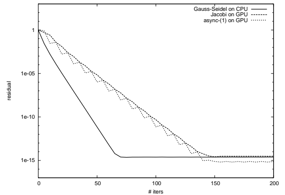
Figure 4: Convergence behavior of test matrix CHEM97ZTZ
