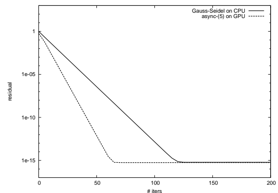
Figure 12: Convergence behaviour of async-(5) for test matrix FV2
