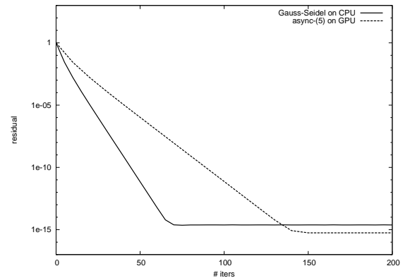
Figure 10: Convergence behavior of async-(5) for test matrix CHEM97ZTZ
