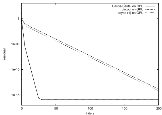
Figure 9: Convergence behavior of test matrix TREFETHEN_2000
