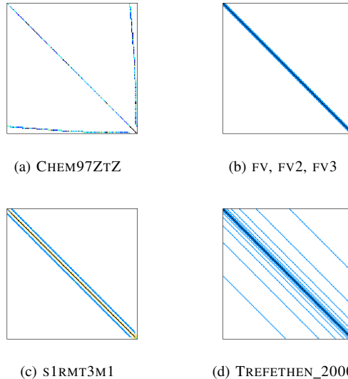
Figure 1: Sparsity plots of test matrices.
