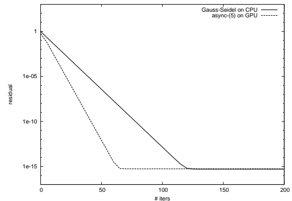
Figure 11: Convergence behavior of async-(5) for test matrix FV1
