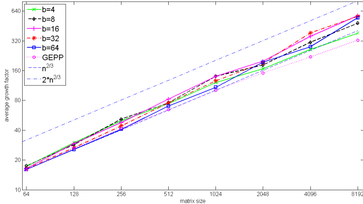
FIG. 3.2. Growth factor g_T of flat tree based CALU for random matrices.
