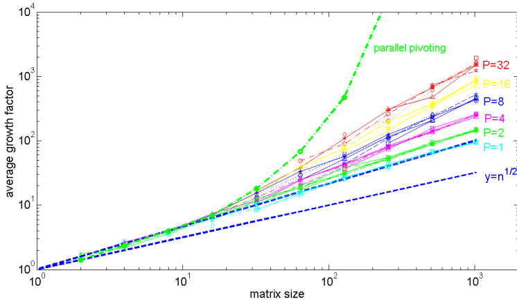
FIG. 4.1. Growth factor of block parallel pivoting for varying block size b and number of processors P .
