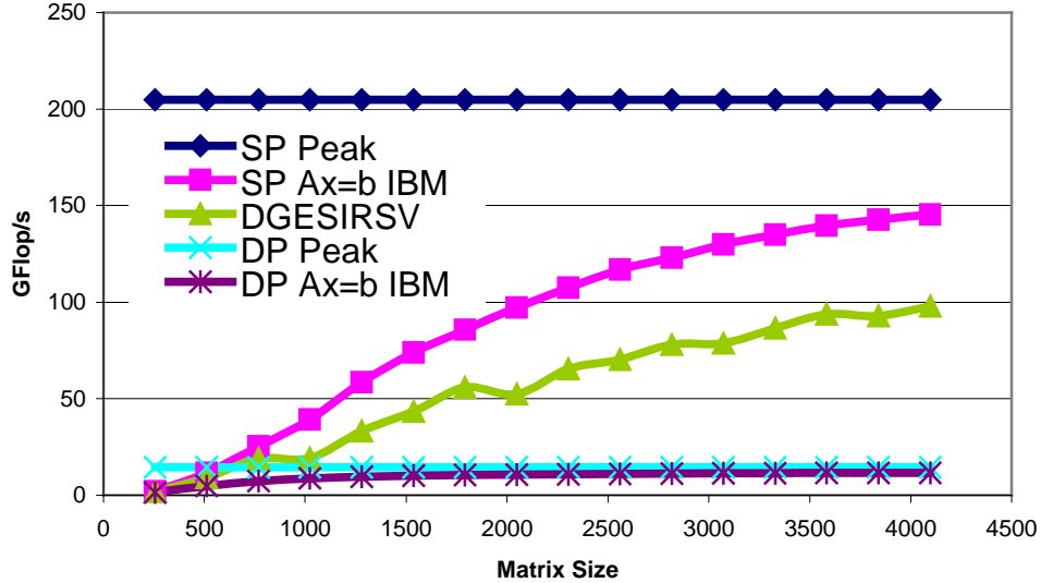
Figure 4: DGESV/DGESIRSV on the IBM Cell Broad Engine.
