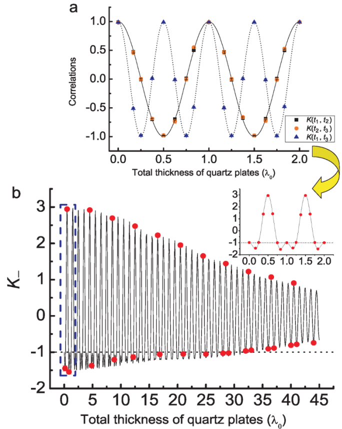
Figure 3 | Violating the LG inequality with K_- . (a) The corresponding values for individual correlations K(t_1, t_2) , K(t_2, t_3) and K(t_1, t_3) to get K_- in the inset of (b). The solid line, dashed line and dotted line are the corresponding theoretical predictions (the solid line and the dashed line completely overlap and only the solid line can be seen). The x axis represents the total thickness of quartz plates between t_1 and t_2 . (b) The envelope evolution of K_- . Red dots represent the experimental results. Solid lines are the theoretical fittings employing equation (3). The dashed line represents the classical limit, -1 . The x axis represents the total thickness of quartz plates between t_1 and t_2 . The inset displays the oscillation between the maximum and minimum in the blue dashed pane (the x axis represents the total thickness of quartz plates between t_1 and t_2 , and the y axis represents K_- ). Error bars correspond to the random fluctuations of each measured coincidence count and the tilt uncertainties of quartz plates. \lambda_0 = 0.78 \mu\text{m} .
