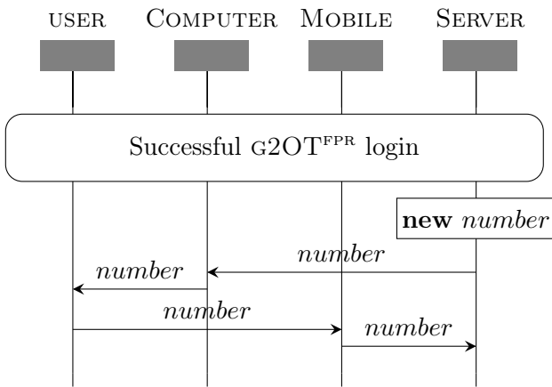
Figure 3.3: g2DT FPR Protocol
