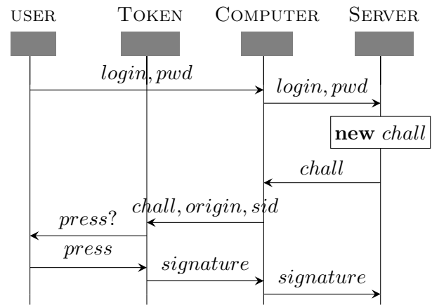
Figure 3.4: U2F Protocol
