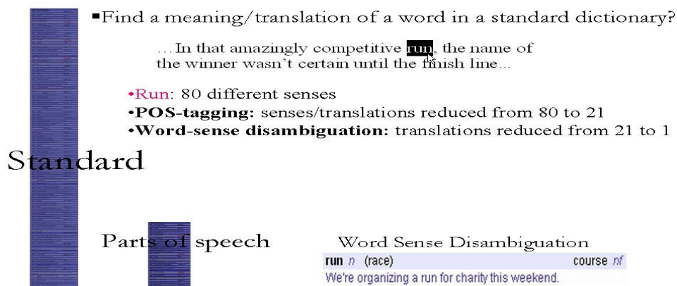
Figure 3: The process of narrowing down the list of possible translations
