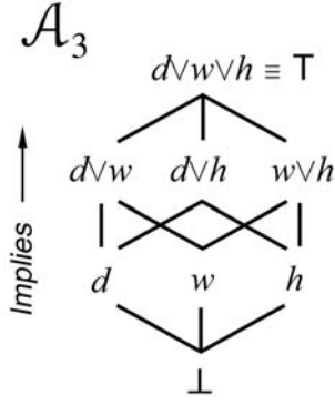
Figure 1: \mathcal{A}_3 is the Boolean lattice formed from three mutually exclusive assertions ordered by the relation ‘ implies ’. The bottom element \perp is the absurdity, which is always false, and the top element \top is the truism, which is always true.
