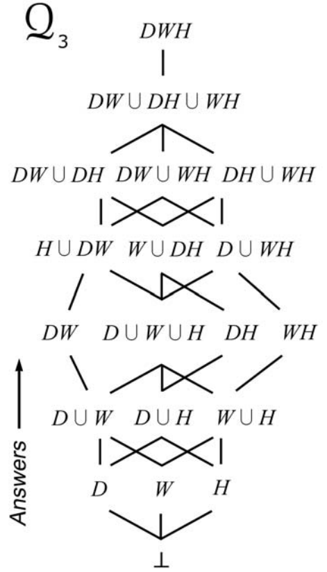
Figure 2: \mathcal{Q}_3 is the free distributive lattice formed from the assertion lattice \mathcal{A}_3 . Questions are ordered by set-inclusion which implements the relation ‘ answers ’.
