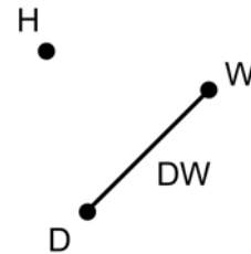
Figure 3: The hypergraph associated with the question H \cup DW = 'Do you or do you not need a hammer?'
