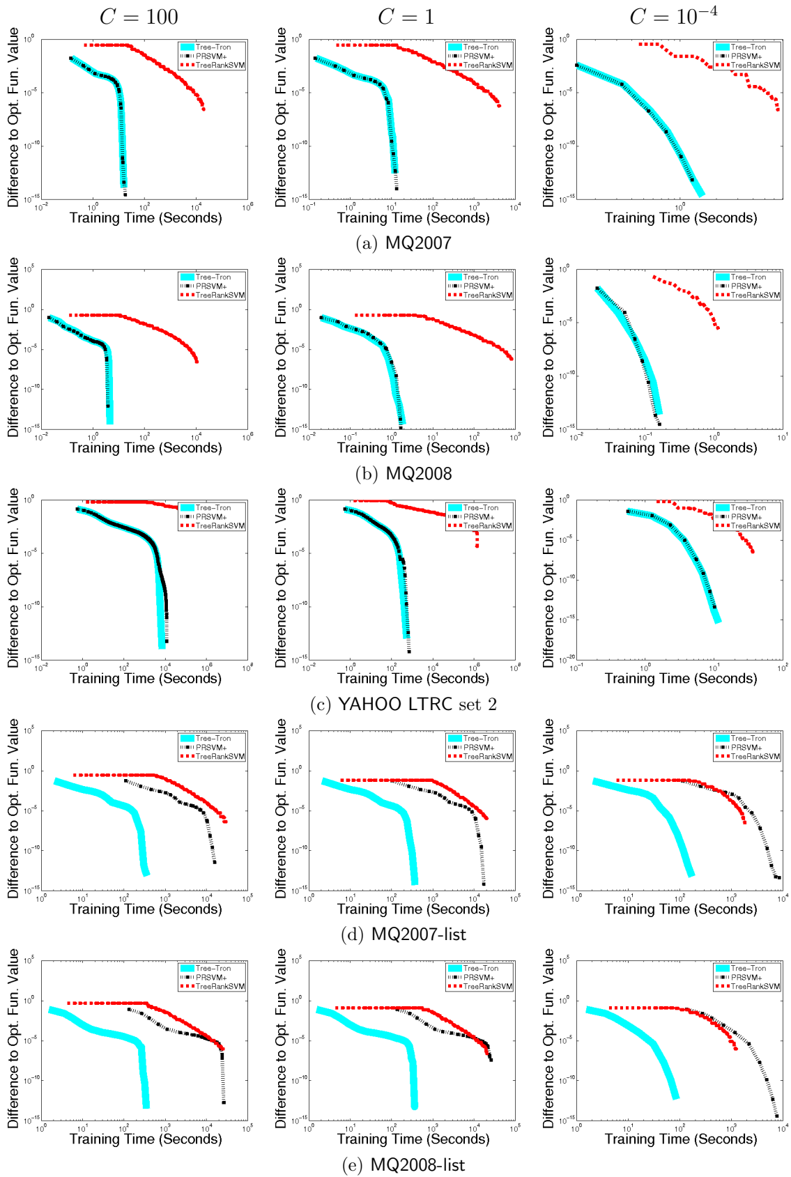
Figure 7: A comparison between different linear rankSVM methods on relative function value with the same C . We set C to be 100, 1 and 10^{-4} .
