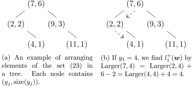
Figure 1: An illustration of using an order-statistic tree to calculate l_i^+(\mathbf{w})
