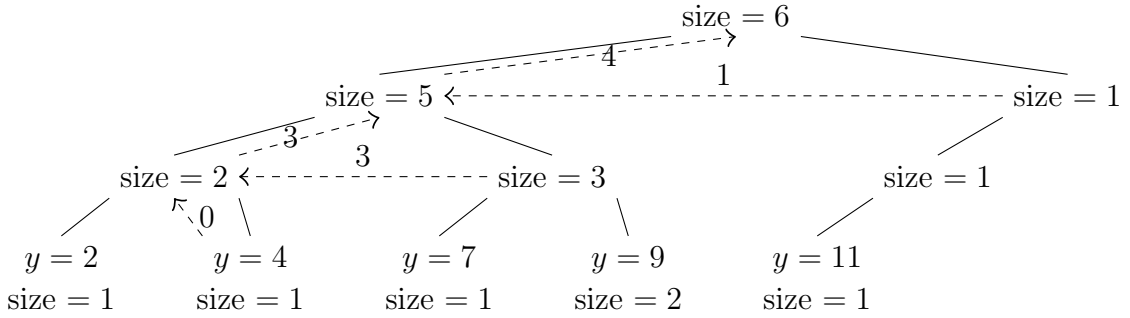
Figure 3: An example of finding l_1^+(\mathbf{w}) when storing y_j in leaf nodes. Note that we assume y_1 = 4 .
