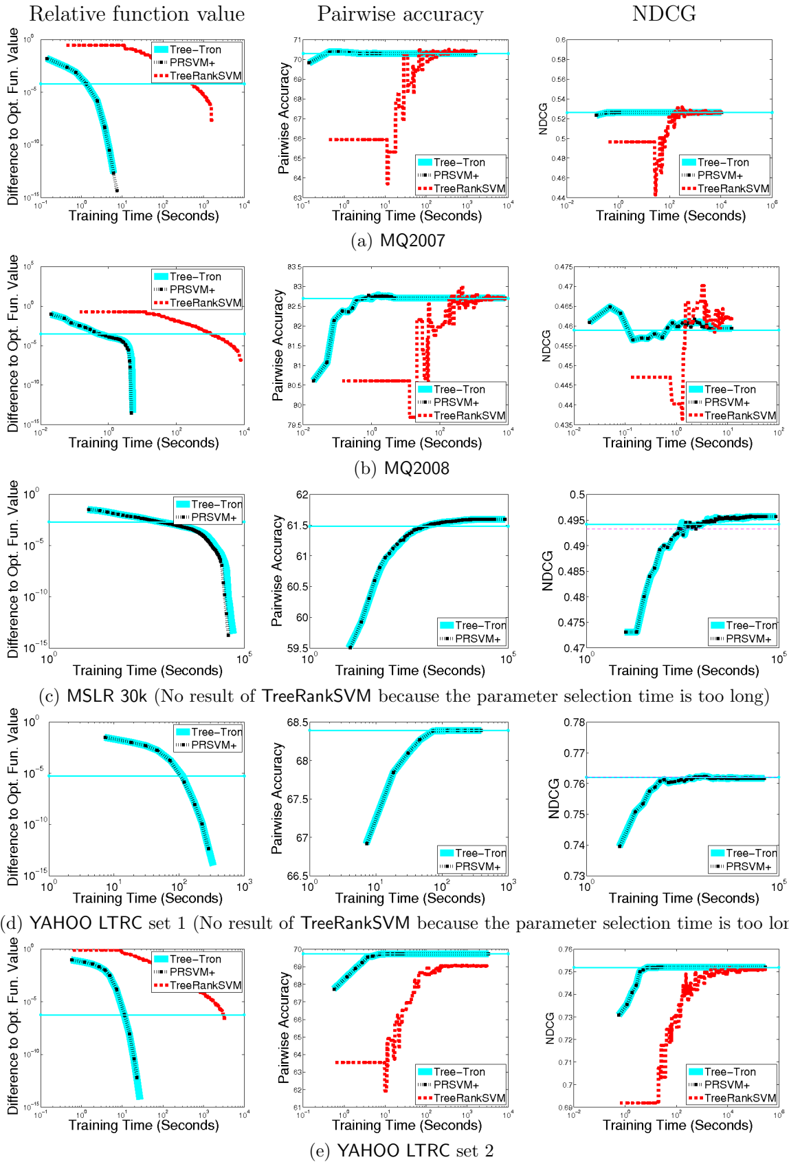
Figure 5: A comparison between different linear rankSVM methods on function values, pairwise accuracy and NDCG. x -axis is in log scale.
