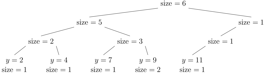
Figure 2: An example of storing y_j in leaf nodes.
