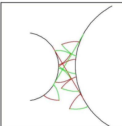
Figure 23: Euler gear, 1767
