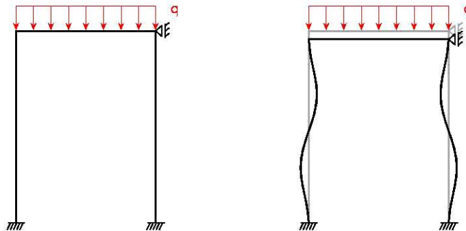
Figure 19: The buckling of a rod
