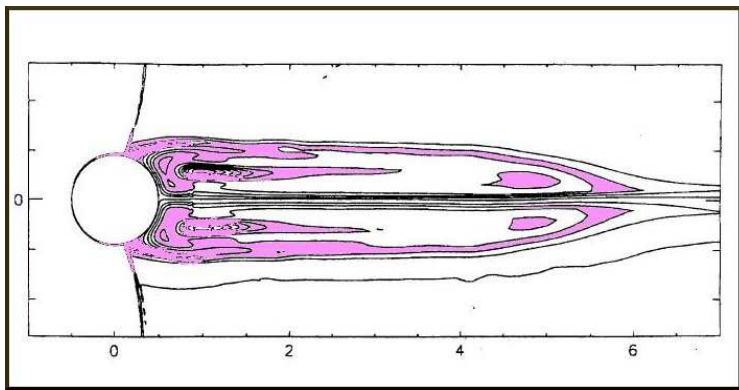
Figure 20: Transonic Euler flow at Mach .85 about a cylinder
