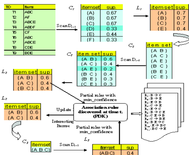
Figure 5. The proposed algorithm mining process from transaction database ( D_{i+1} ).
