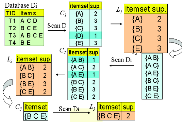
Figure 4. A priori mining process.
