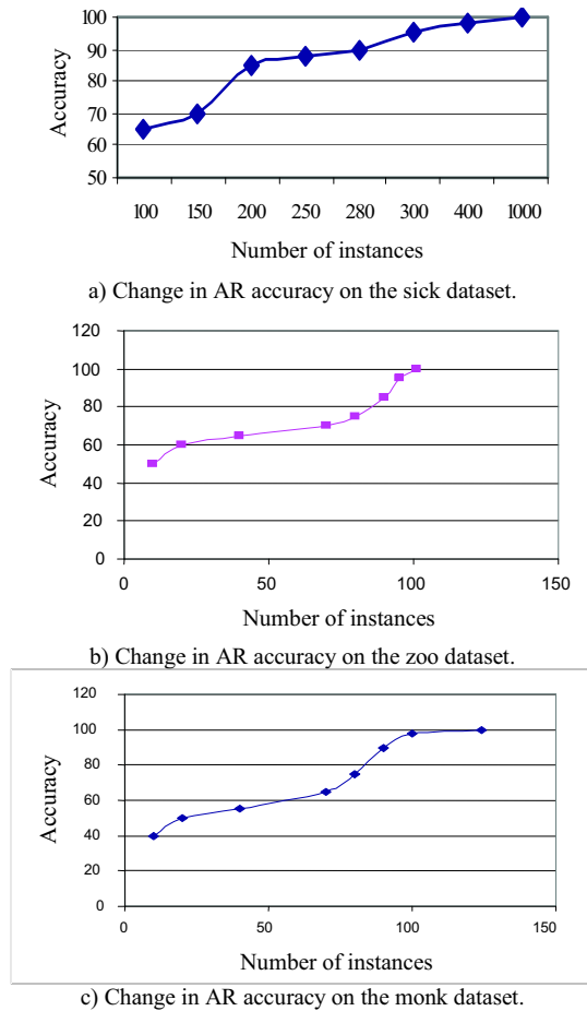
Figure 6. Sick, zoo and monk datasets experiment.
