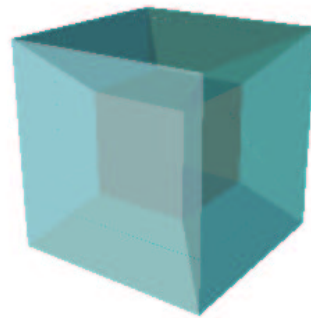
Hypercube's central projection onto the 3D space.
