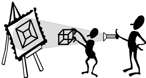
Projecting a cube on a plane (central projection).
