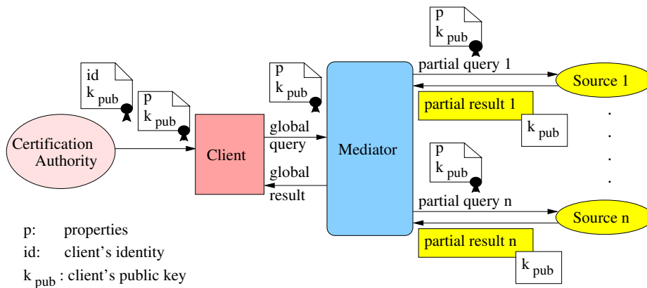
Fig. 2. A credential-based secure mediated information system
