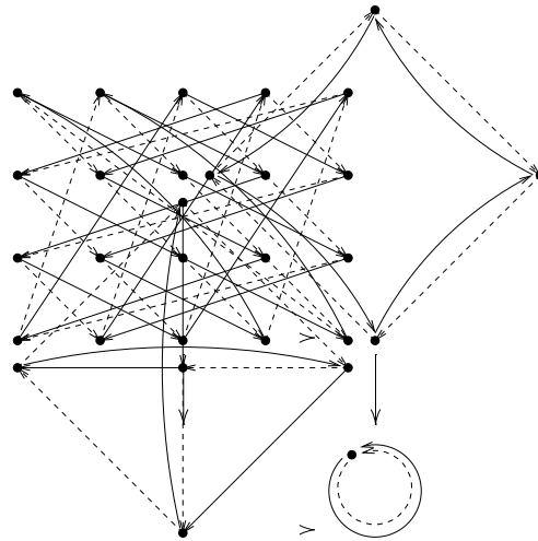
Figure 7: A pullback of two covering projections.
