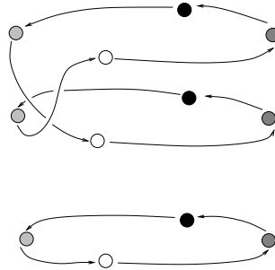
Figure 2: An eight-cycle covering a four-cycle.
