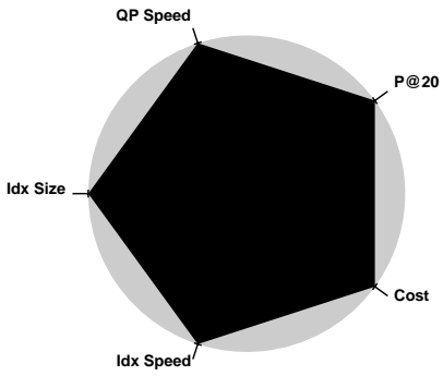
All-Round Best
