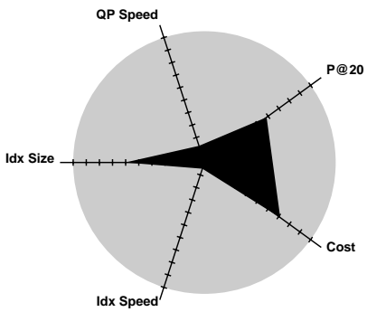
ACSys - acsys8lw0_pr10
