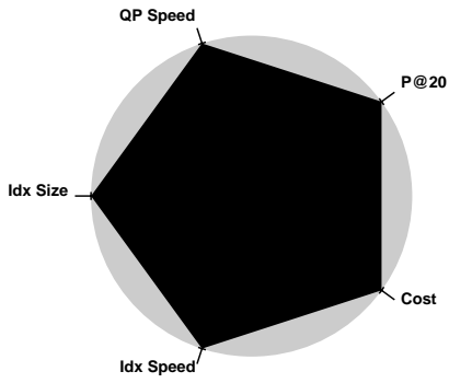
All-Round Best
