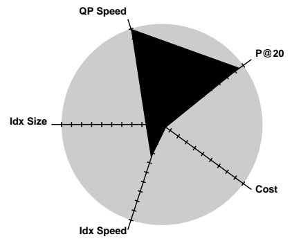
AT&T - att99vlcm
