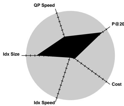
Fujitsu - fl8wlinsr
