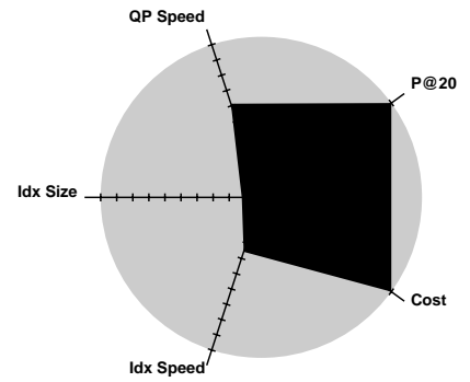
UWaterloo - uwmt8lw0
